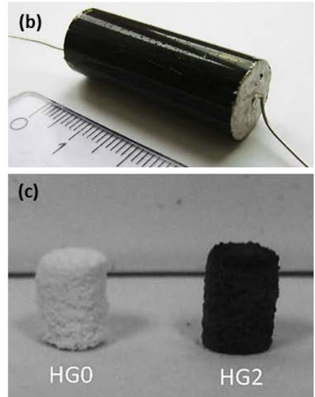
Fig. 3. (a) Schematic illustration of a layer-by-layer fabrication of a 3D structure using the powder bed technology, [55] (b) photo of printed carbon nanofiber nanocomposite sample prepared for volume electrical measurements, [57] and (c) porous structures (cylinders) of nanocomposites containing 0 wt.% GO (HG0) and 0.2 wt.% GO (HG2) fabricated by powder-bed 3DP. [58]
