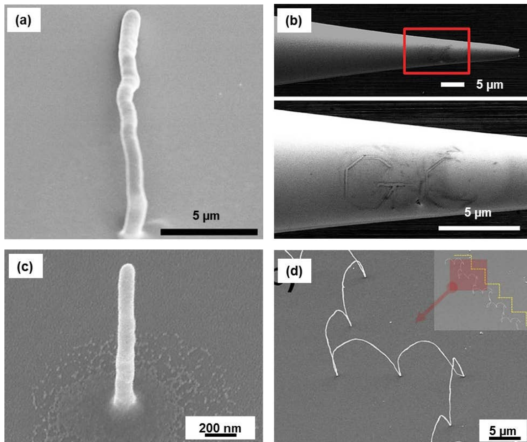
Fig. 25. SEM images of representative 3D printed structures using nanomaterial solutions: (a) an e-jet printed nanopillar fabricated using copper nanoparticle suspension (30 wt.%) mixed with n-tetradecane (1:1 weight ratio), [97] (b) rGO patterns e-jet printed on the sidewall of a glass microcapillary as a substrate fabricated using rGO nanoparticles dispersed in DMF. The capillary nozzle has a cone geometry with an internal diameter of 5 \mu\text{m} and a curvature radius of 50-65 \mu\text{m} , [95] (c) an e-jet printed gold nanopillar with diameter of \sim 50 nm and height of \sim 850 nm made of gold nanoparticle solution ( \sim 0.1 vol.% in a mixed solution of n-tetradecane and cyclododecene (50:1 wt./wt.)), [98] and (d) a zigzag rGO nanoarch with a constant arch width ( r = 400 nm) fabricated via the meniscus-guided growth 3DP using an aqueous suspension of GO nanosheets, [99]
