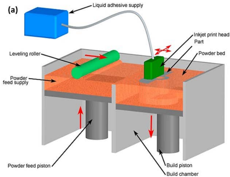
Fig. 3. (a) Schematic illustration of a layer-by-layer fabrication of a 3D structure using the powder bed technology, [55] (b) photo of printed carbon nanofiber nanocomposite sample prepared for volume electrical measurements, [57] and (c) porous structures (cylinders) of nanocomposites containing 0 wt.% GO (HG0) and 0.2 wt.% GO (HG2) fabricated by powder-bed 3DP. [58]
