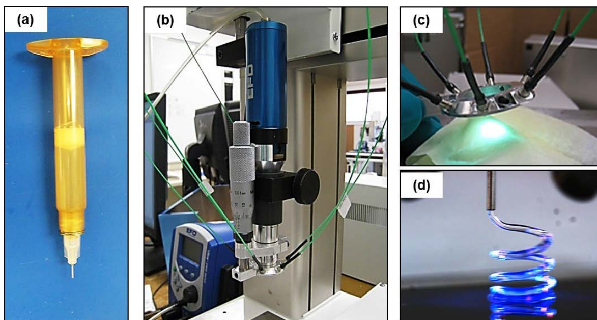
Figure 2. (a) a 3 CC syringe containing a UV-curable material, (b) the deposition setup with inserted syringe and pressure piston, mounted on the computer-controlled robot, (c) UV light delivery system consisting of six fiber optics showing UV radiation emitted (mounted on the robot in (b)), and (d) image of a microspring deposition using a UV-curable ink.
