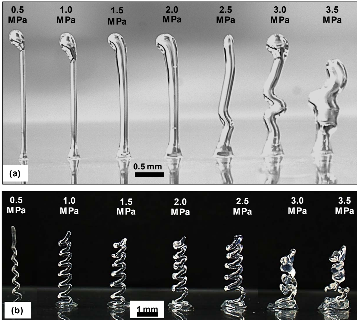
Figure 8. UV-3DP fabrication of (a) vertical filaments and (b) freeform microsprings at different extrusion pressures and a constant deposition speed of \sim 0.5 mm/s using an extrusion nozzle of 150\mu\text{m} -internal diameter and the UV-PU resin, NEA 123T.
