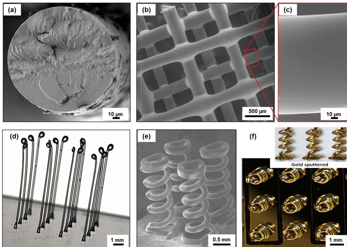
Figure 10. Optical and SEM images of several representative microstructures fabricated using the UV-3DP technique: (a) a typical fabricated filament cross-section, (b) a 3D periodic 4-layer scaffold, (c) higher magnification of (b), (d) a network of 16 vertical microrods, (e) a network of 4 nanocomposite microsprings, (f) a network of 9 gold-sputtered microsprings electrodes.
