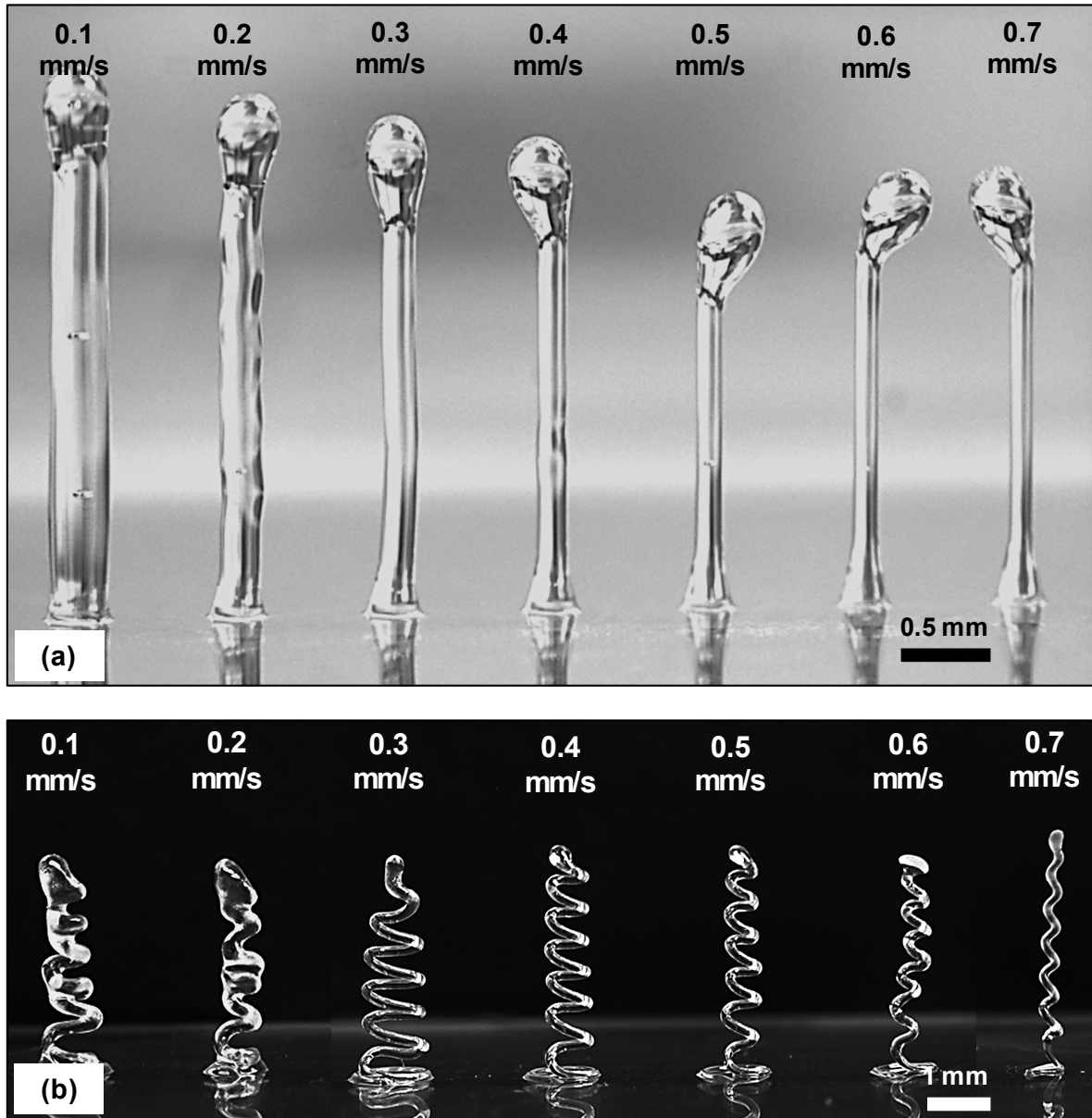
Figure 7. UV-3DP fabrication of (a) vertical filaments and (b) freeform microsprints at different deposition speeds and a constant extrusion pressure of \sim 1 MPa using an extrusion nozzle of 150\mu\text{m} -internal diameter and the UV-PU resin, NEA 123T.
