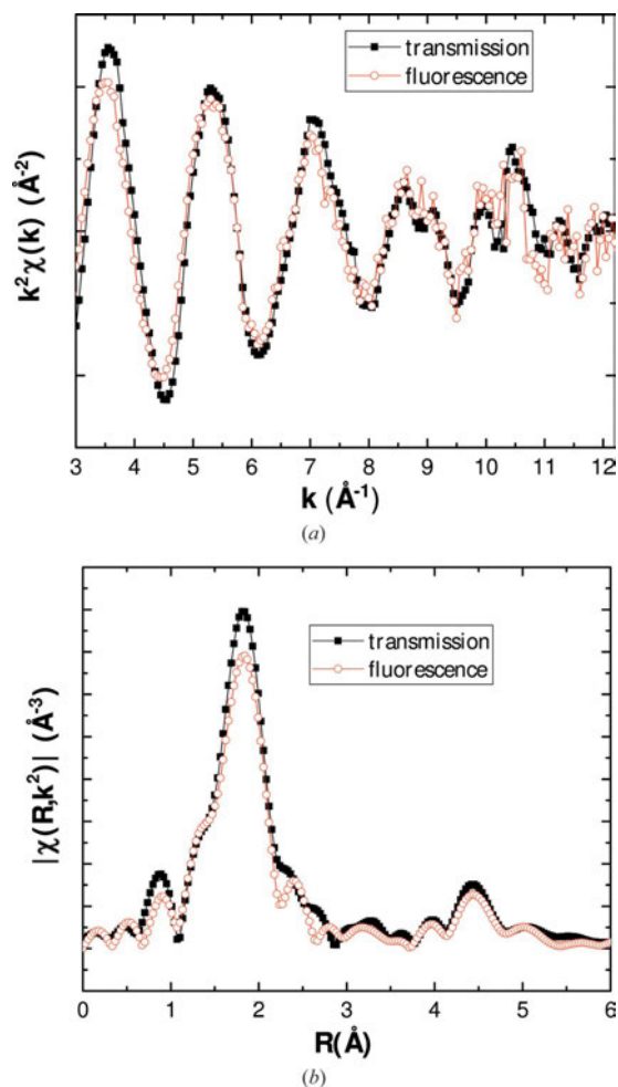
Figure 15 (a) Experimental k^2\chi(k) spectra and (b) Fourier transform modulus of \text{ThF}_4 measured at room temperature in transmission and fluorescence. Note that the fluorescence spectrum was not corrected for self-absorption effects.
