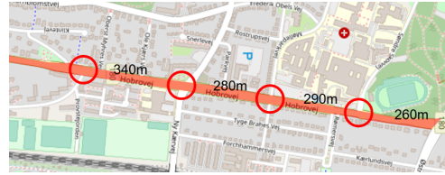
Fig. 5. Intersections optimized by UPPAAL STRATEGO at Hobrovej, Aalborg
