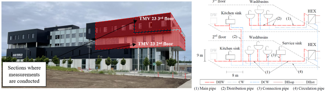
Fig. 2. To the left is TMV 23, with highlighted sections where measurements are conducted. To the right is a sketch (not to scale) of the DHW systems. The measured draw-off points are marked with bold.
