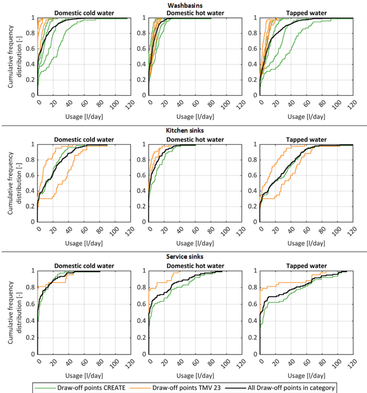
Fig. 5. Daily usage of hot, cold, and tapped water from washbasins, kitchen sinks and cleaning sinks in CREATE and TMV 23.
