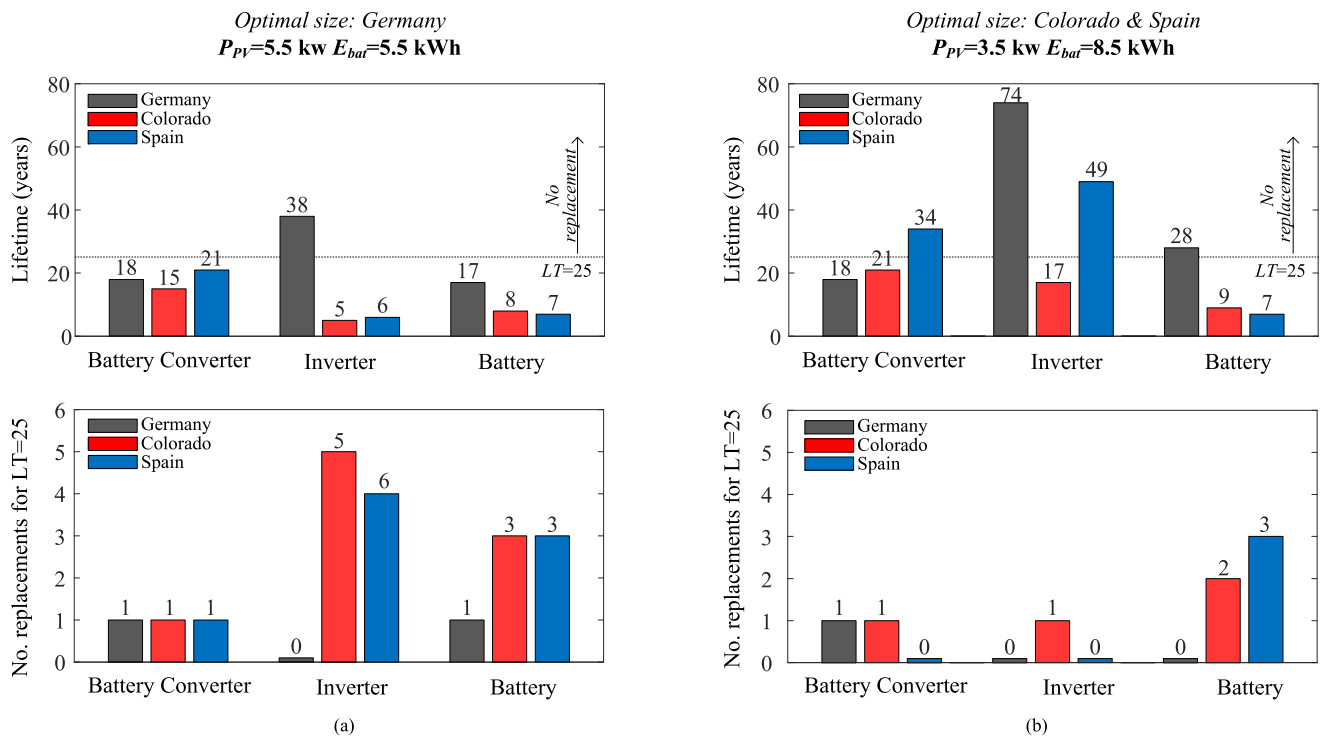
FIG. 13. Lifetime of reliability-critical components and number of replacement during the project lifetime LT of 25 years for: (a) Case 1, where PV and battery sizes are set to P_{pv}=5.5 kW E_{bat}=5.5 kWh representing the optimal size for mission profile in Germany and, (b) Case 2, where PV and battery sizes are set to P_{pv}=3.5 kW E_{bat}=8.5 kWh representing the optimal size for mission profiles in Colorado and Spain.
