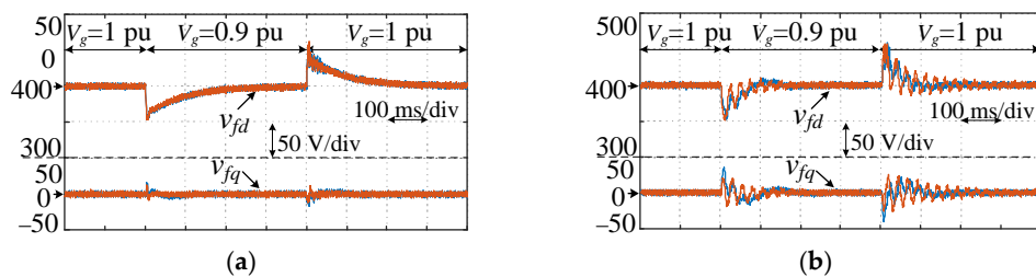
Figure 9. Time-domain simulations showing the system response for 10% voltage sag at grid voltage under different power levels ( P = 0.25P_n (orange) and P = 0.75P_n (blue)). (a) SCR = 5; (b) SCR = 1.67.
