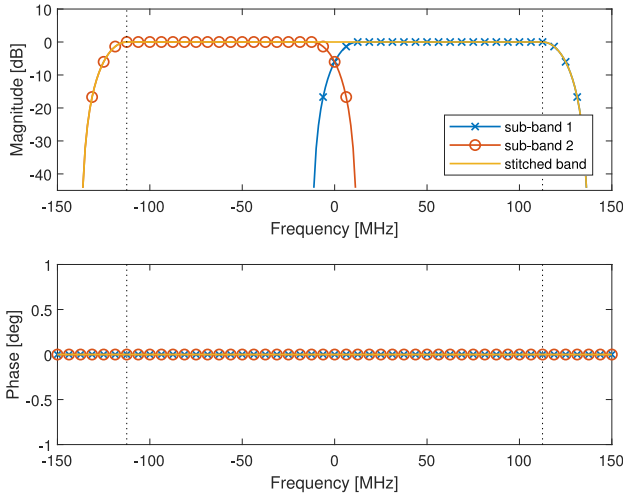
FIGURE 2. (Top) the magnitude and (bottom) the unwrapped phase (normalized at the center frequency) of the frequency response. The black dotted lines indicate the 225 MHz distortion-free bandwidth.
