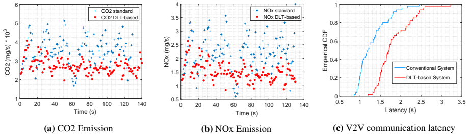
Fig. E.6: Performance Evaluation. (a) and (b): The \text{CO}_2 and \text{NO}_x emission generated in standard and DLT based systems; (c) Communication latency between standard and Blockchain-based system.
