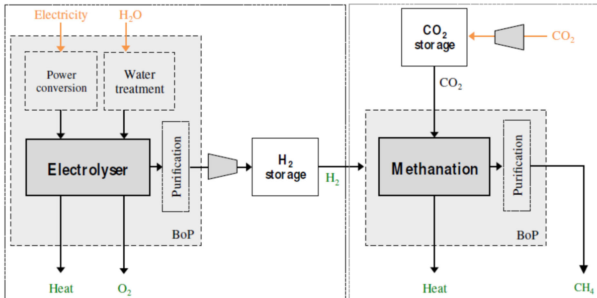
Figure 5. Overview of a P2G plant (Leuwen & Zauner, 2018)
