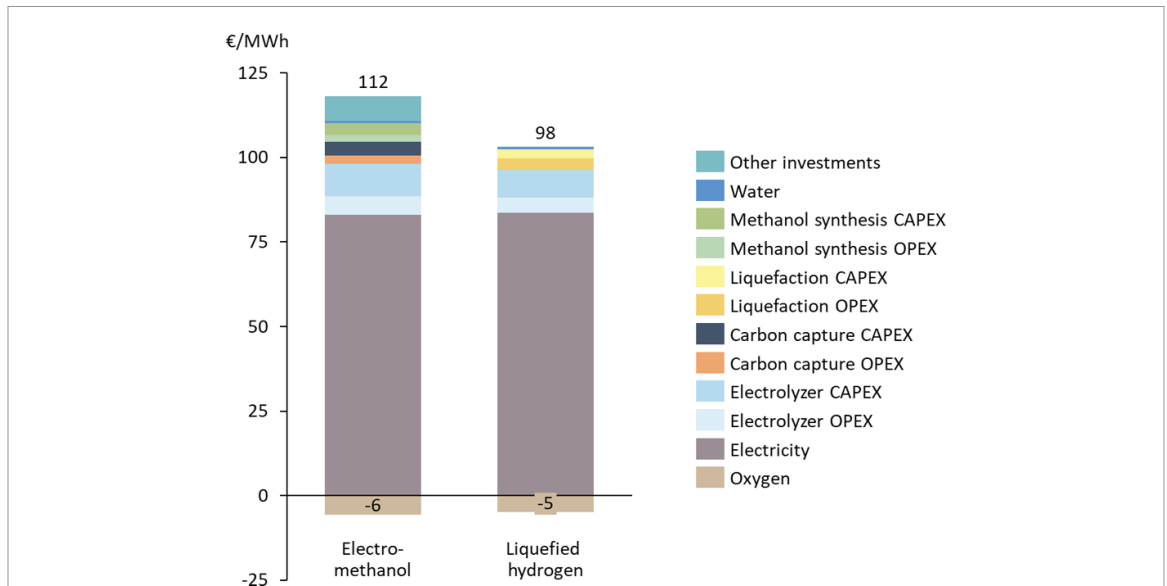
Figure 4. Production costs for e-methanol and liquefied electrolytic hydrogen showing the different component costs, using base values (long-term) from the literature review. All data used in the calculations are presented in table 7. In this study, revenues are not included in the harmonized fuel production costs but as an illustration of the effect a revenue can have, the potential cost reduction of being able to sell high-purity oxygen at 50 €/tO 2 is shown. Acronyms used: CAPEX capital expenditures, OPEX operational expenditures.
