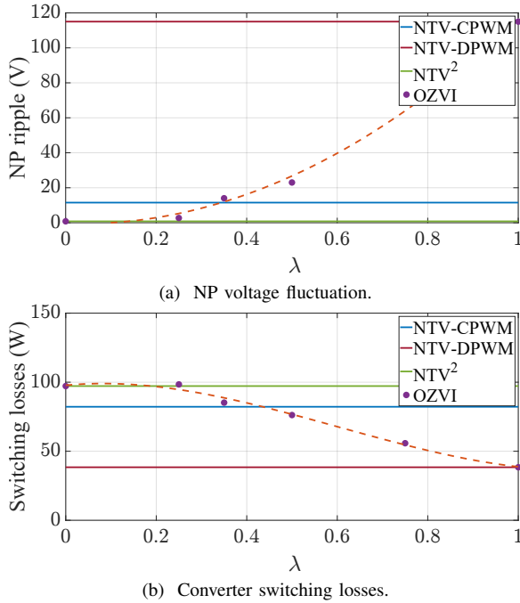
Fig. 8: Comparison of the conventional control methods and proposed OP-ZVI method for high modulation index ( I = 100 A, m_a = 0.9 ) and low frequency (10 Hz).
