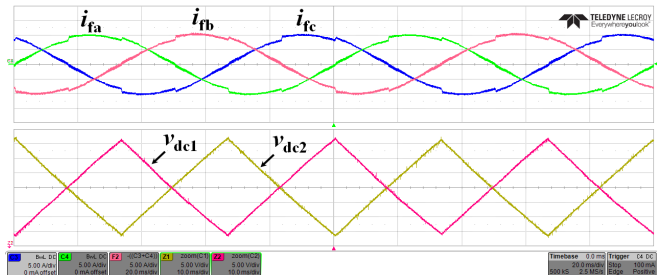
(a) For \lambda = 1 (NTV-DPWM).
