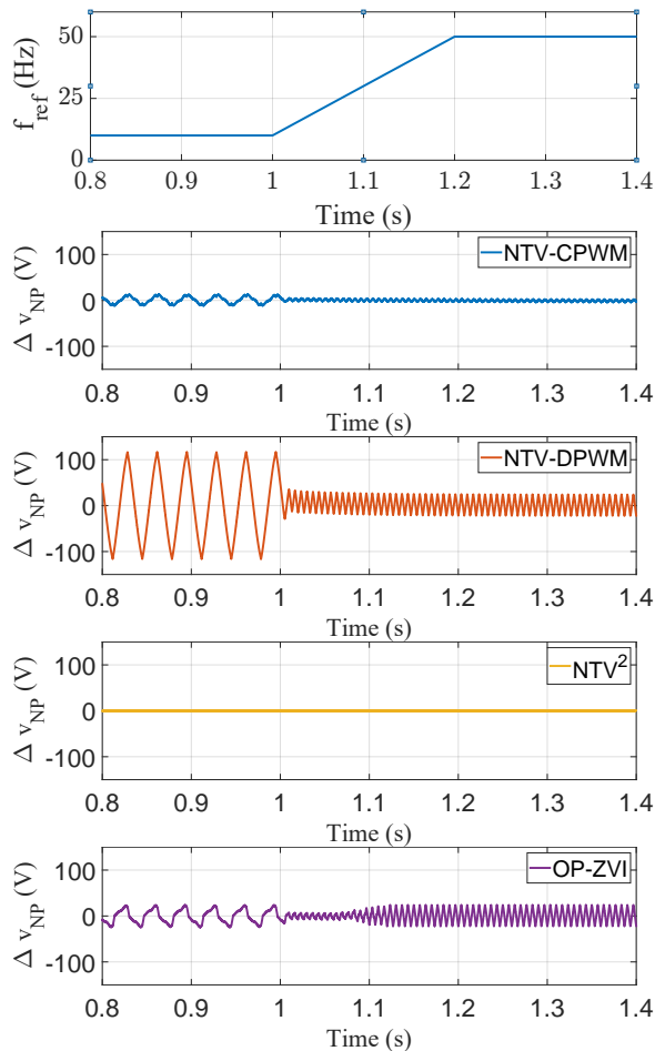
Fig. 11: Comparison of the NP voltage fluctuation for ZVI methods during f_{ref} change from 10 \rightarrow 50 Hz ( m_a = 0.9 ). Load is constant.
