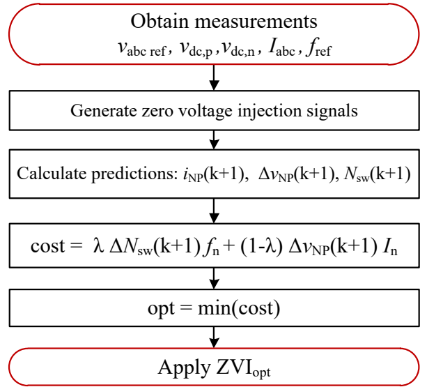
Fig. 4: Workflow of the proposed OP-ZVI method.
