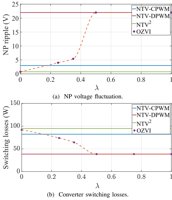
Fig. 7: Comparison of the conventional control methods and proposed OP-ZVI method for high modulation index ( I = 100 A, m_a = 0.9 ) and high frequency (50 Hz).
