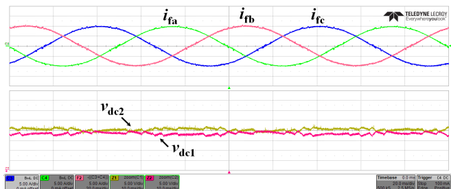
(c) For \lambda = 0.5 (OP-ZVI).
