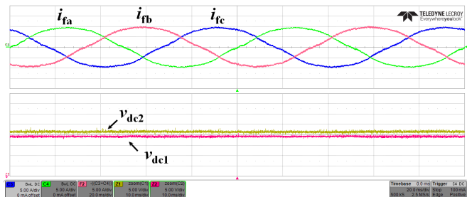
(b) For \lambda = 0 (NTV 2 ).
