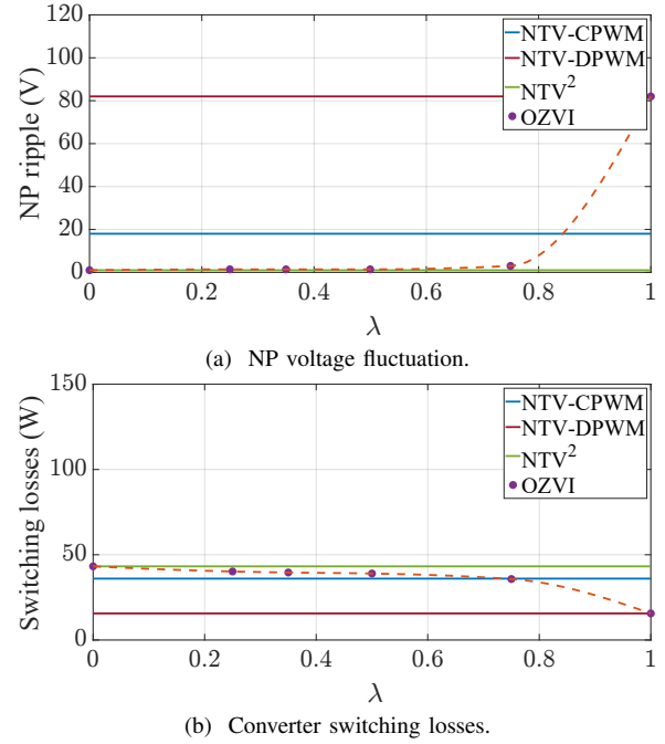
Fig. 10: Comparison of the conventional control methods and proposed OP-ZVI method for low modulation index ( I = 55 A, m_a = 0.5 ) and low frequency (10 Hz).
