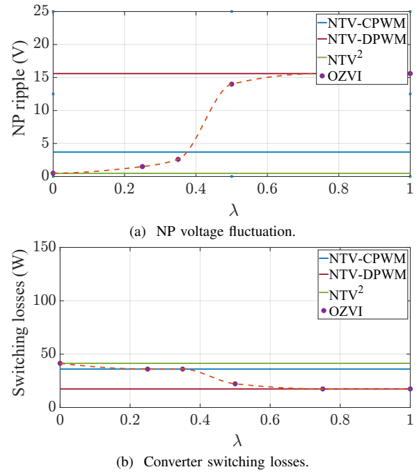
Fig. 9: Comparison of the conventional control methods and proposed OP-ZVI method for high modulation index ( I = 55 A, m_a = 0.5 ) and high frequency (50 Hz).
