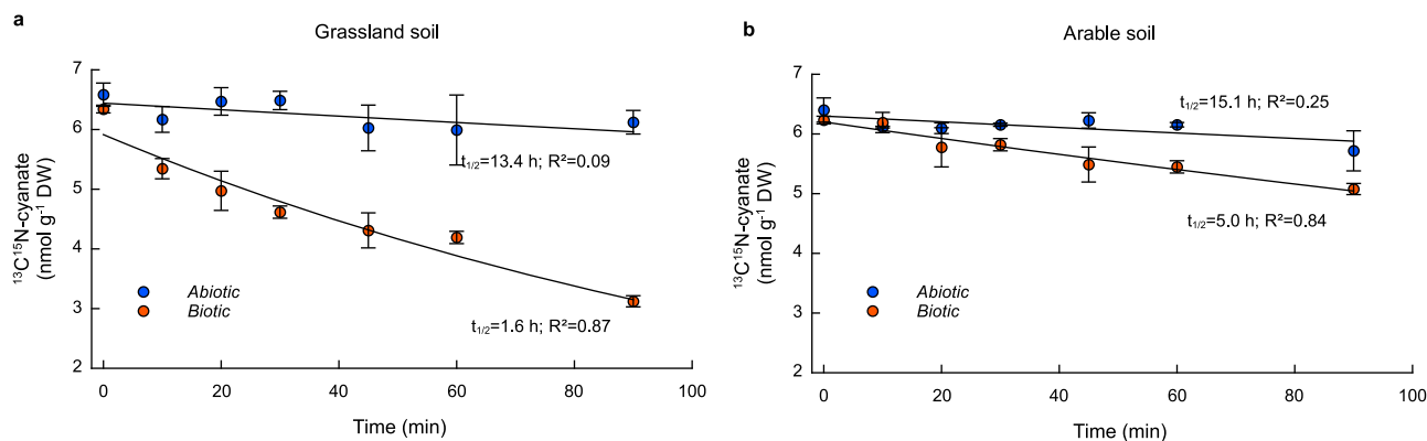
Fig. 3 Dynamics of soil ^{13}\text{C}^{15}\text{N} -cyanate consumption in two contrasting neutral soils ( \text{pH} = 7.4 ) (“tracer experiment”). ^{13}\text{C}^{15}\text{N} -cyanate was added to a sterile (i.e., abiotic control) and non-sterile (a) grassland soil and (b) arable soil, and incubations were stopped after 0, 10, 20, 30, 45, 60, and 90 min. To obtain biotic cyanate consumption over time, the non-sterile samples were corrected for abiotic loss of cyanate derived from the sterile samples. Dynamics of cyanate consumption over time for the corrected non-sterile soils and sterile soils were described by fitting a first-order exponential decay curve and the exponential coefficient was used to calculate half-life ( t_{1/2} ) of the ^{13}\text{C}^{15}\text{N} -cyanate pool. Shown are average values \pm 1\text{SE} ( n = 3 ).
