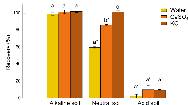
Fig. 1 Comparison of extractants for determination of soil cyanate concentration. Cyanate recovery was assessed by spiking the extraction solution with potassium cyanate (final concentration of 15 nM). Three extractants (water, 10 mM Calcium sulfate ( \text{CaSO}_4 ), and 1 M Potassium chloride (KCl)) were tested for three soils: an alkaline grassland soil (soil pH = 8.3), a pH-neutral mixed forest soil (soil pH = 7.0) and an acidic grassland soil (soil pH = 4.3). Letters denote significant differences between extractants within each soil type (one-way ANOVA followed by Tukey's HSD test, \alpha = 0.05 ). Asterisks indicate significant differences between added and recovered cyanate ( t test, \alpha = 0.05 ). Shown are average values \pm 1 SE ( n = 4 ).
