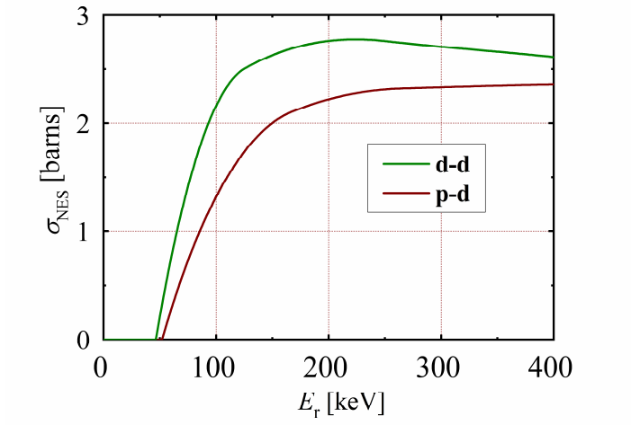
Figure 2 Cross sections of deuteron-deuteron and proton-deuteron NES as a function of the relative energy of reactants.
