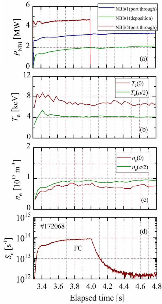
Figure 3 Time evolution of the deuterium plasma discharge (shot no. #172068). (a) neutral beam heating powers for injectors NBI#1, and 5; (b) electron temperatures at r = 0 and a/2 ; (c) electron density at r = 0 and a/2 ; (d) neutron generation rate detected by the fission chamber (FC).
