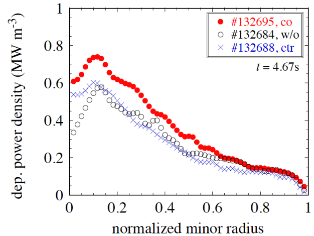
Fig. 5 Radial profiles of NBI deposition power density imparted to the ions, analyzed by TR-snap code at t = 4.67 s in the co-ECCD, counter-ECCD, and no ECCD discharges.
