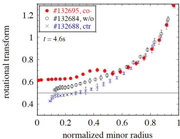
Fig. 2 Radial profiles of rotational transform diagnosed by MSE measurements at t = 4.6 s in the co-ECCD, counter-ECCD, and no ECCD discharges.
