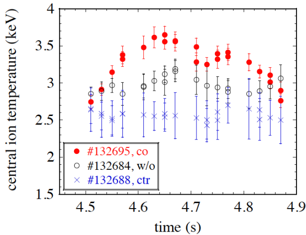
Fig. 4 Time evolutions of central ion temperature in the co-ECCD, counter-ECCD, and no ECCD discharges. The results were obtained by temporal averaging of each set of three neighboring data points in the original data.
