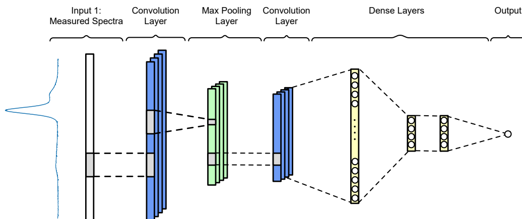
Figure 1. The neural network architecture used in this work. It is made of one convolutional layer (6 filters of size 40), one max pooling layer (size 8), one convolutional layer (4 filters of size 20), one dropout layer (rate 0.5), two subsequent flatten layers (4 neurons) and a final neuron for regression. Apart from the output neuron that uses the identity activation functions, all other layers use the ReLU (Rectified Linear Unit) activation function.
