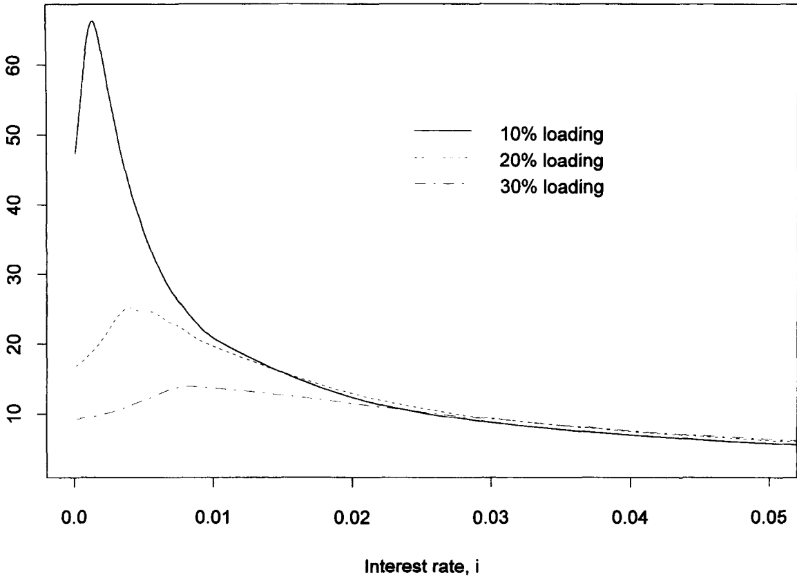
Fig. 4. Exponential claims, standard deviation of T(u) .
