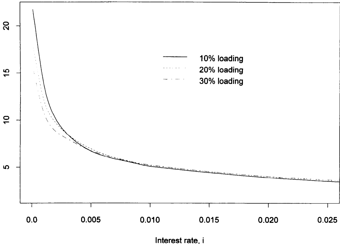
Fig. 6. Pareto (2,1) claims, standard deviation of T(0) .
