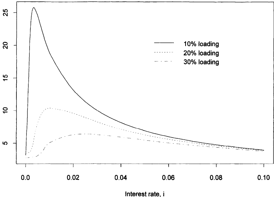
Fig. 11. Exponential claims, standard deviation of L(u) .
