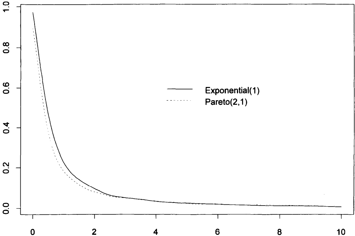
Fig. 7. Densities of T(0) when i = 0.001 .
