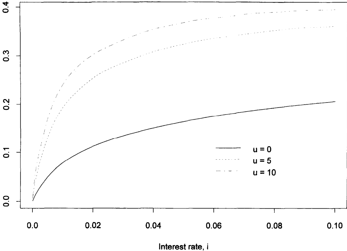
Fig. 2. Pareto (2,1) claims and 10% loading, \phi(u) .
