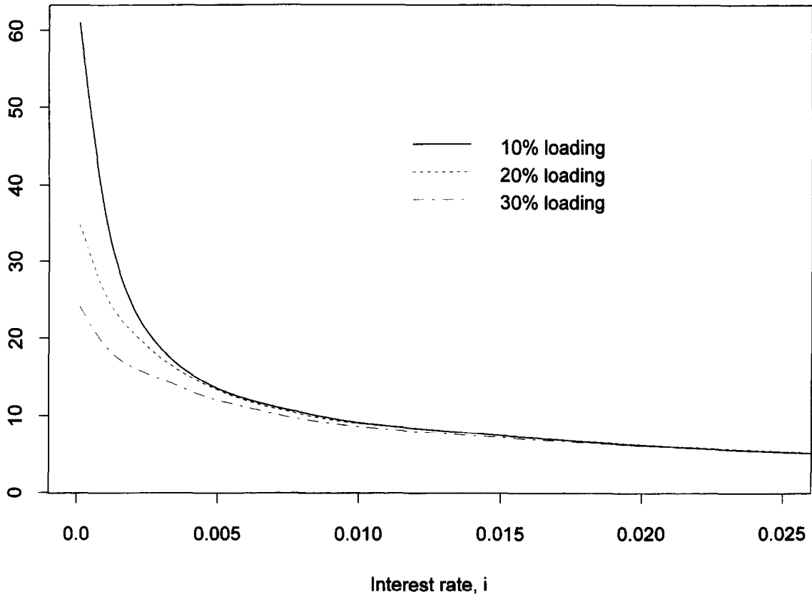
Fig. 5. Pareto (2,1) claims, E(T(0)) .
