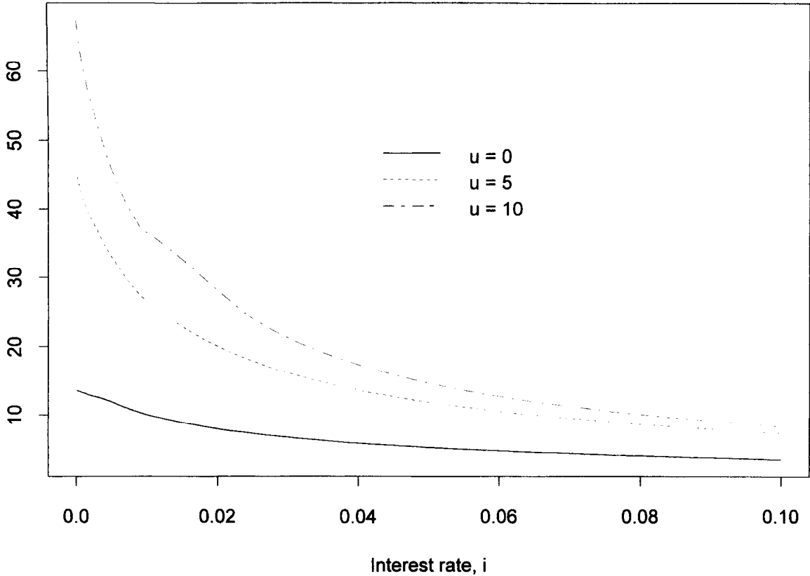
Fig. 12. Pareto (2,1) claims and 20% loading, E(L(u)) .
