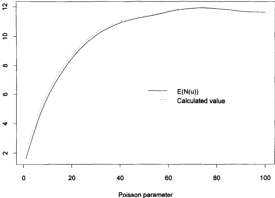
Fig. 8. Exponential claims, E(N(u)) .
