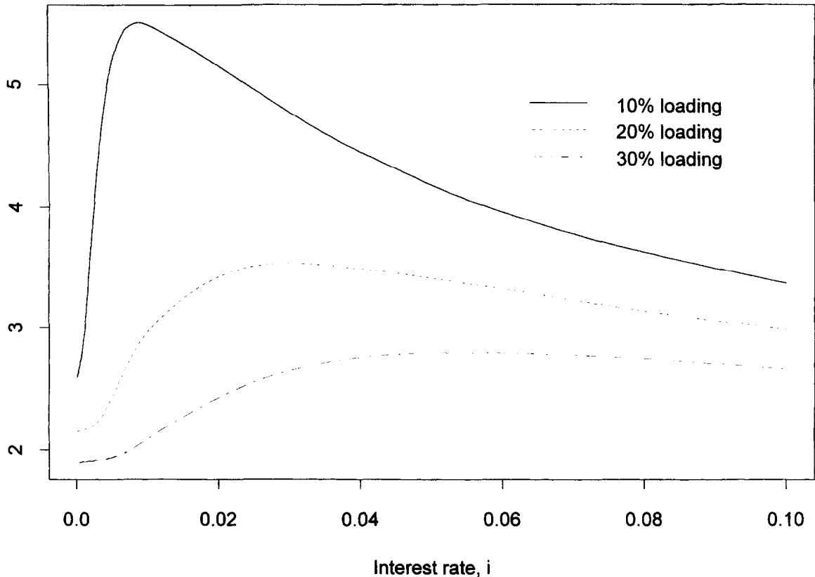
Fig. 10. Exponential claims, E(L(u)) .
