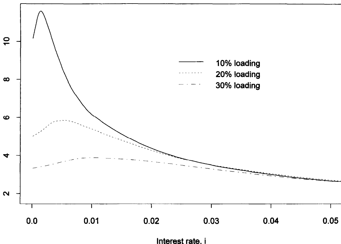
Fig. 3. Exponential claims, E(T(u)) .
