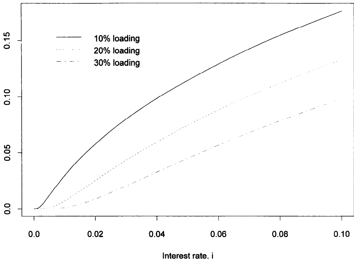
Fig. 1. Exponential claims, \phi(u) .
