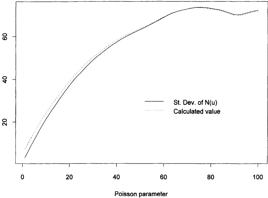
Fig. 9. Exponential claims, standard deviation of N(u) .
