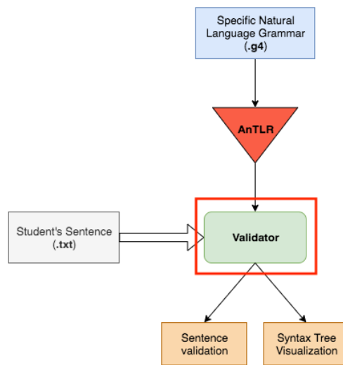
Figure 9: Excerpt of the system architecture - Sentence Validator.
