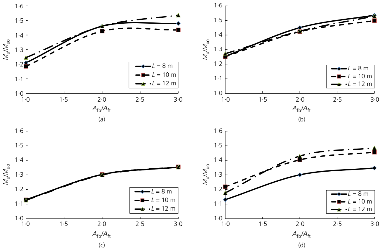
Figure 8. Effect of steel flange area ratio on the ultimate resistance of externally prestressed steel–concrete composite beams (PCB) (SA): (a) group A under concentrated loads; (b) group A under distributed loads; (c) group B under concentrated loads; (d) group B under distributed loads
