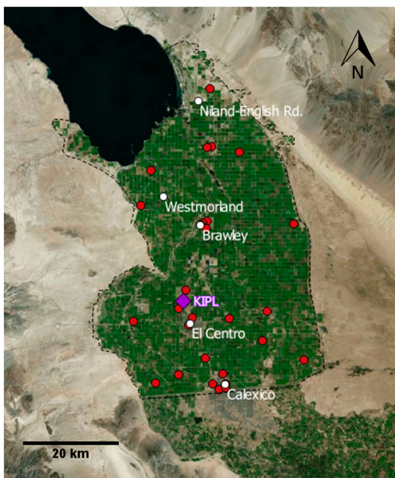
Figure 1. Map of the study area: Particulate matter (PM) mass concentration of particles less than 10 micrometers aerodynamic diameter (PM 10 ) and PM mass concentration of particles less than 2.5 micrometers aerodynamic diameter (PM 2.5 ) ambient air concentration measurement site locations ( white dots ), Identifying Violations Affecting Neighborhoods (IVAN) PM 2.5 data site locations ( red dots ), and the Imperial County Municipal Airport National Weather Service meteorological site location (KIPL) ( purple diamond ). The black dashed line surrounding the Imperial Valley is used to mask the MAIAC AOD fields to retain pixels only within the valley.
