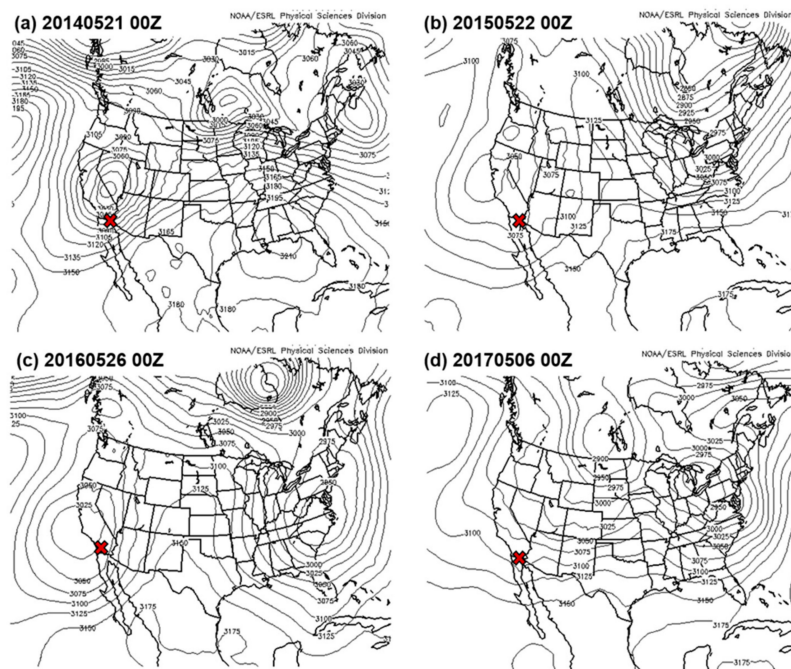
Figure 3. The 700 mb geopotential height fields (meters) from the North American Regional Reanalysis [28] for four west-southwesterly (WSW) high wind events affecting the Imperial Valley. The red X on each panel is the approximate location of valley. Plots were created from the NARR plotting website operated by NOAA/OAR/ESRL PSD, Boulder, Colorado, USA ( https://www.esrl.noaa.gov/psd/data/gridded/data.narr.html ).
