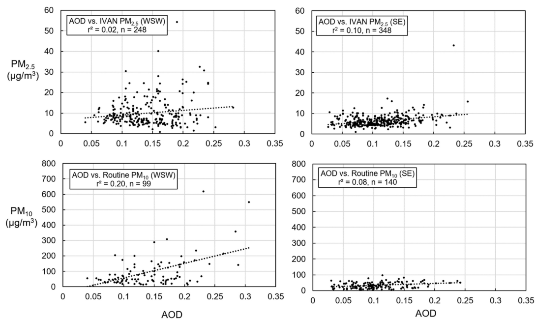
Figure 10. Scatterplots and regression statistics of paired MAIAC AOD and measured PM concentrations at overpass hour; (top left) AOD versus IVAN PM2.5 for the WSW set, (top right) AOD versus IVAN PM2.5 for the SE set, (bottom left) AOD versus routine PM10 for the WSW set, and (bottom right) AOD versus routine PM10 for the SE set.
