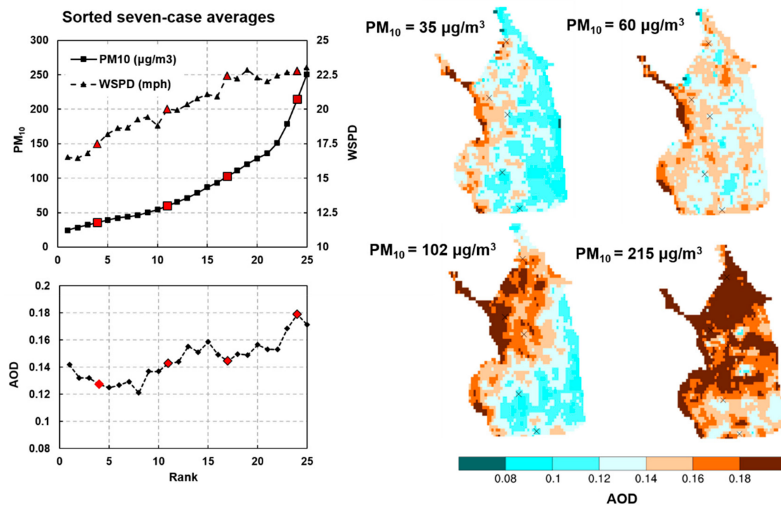
Figure 12. Left: Seven-case running average Brawley-Niland PM 10 concentrations for events comprising the WSW set, sorted lowest to highest (solid-squares, upper left ), and corresponding seven-case running averages for average wind speed at KIPL (dashed-triangles, upper left ) and valley-averaged AOD (dashed-diamonds, lower left ). Right: spatial plots of seven-case running average AOD fields for four representative points on left-hand plot of successively higher PM 10 indicated by red, larger symbols on the left panel. The “x” symbols on right panel are the locations of routine PM 10 sites.
