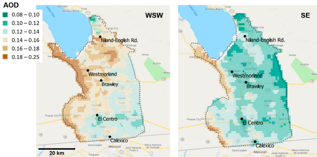
Figure 6. Average multi-angle implementation of atmospheric correction (MAIAC) aerosol optical depth (AOD) fields within the Imperial Valley (dotted line) for the WSW (left) and SE (right) sets. Fields constructed by averaging AOD fields over the cases comprising each respective set ( n = 31 for WSW, n = 47 for SE, see Table 2).
