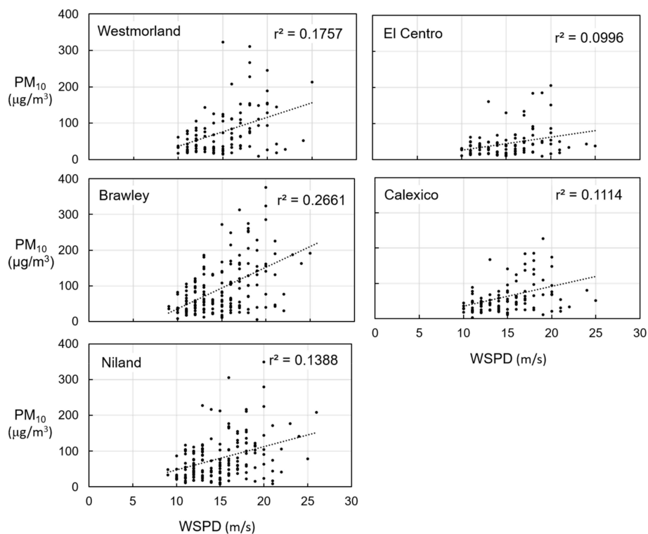
Figure 4. Daily averaged beta-attenuation monitors (BAMS) PM10 concentrations versus daily-averaged wind speed at KIPL for the selected springtime WSW wind events in the Imperial Valley. The coefficient of determination ( r^2 ) of the plotted best-fit regression line is indicated on each panel. Data comprise 165 days between 2013 and 2019 for Brawley and Niland, and 104 days between 2016 and 2019 for Calexico, El Centro, and Westmorland. Criteria of event selection is given in Section 2.3.
