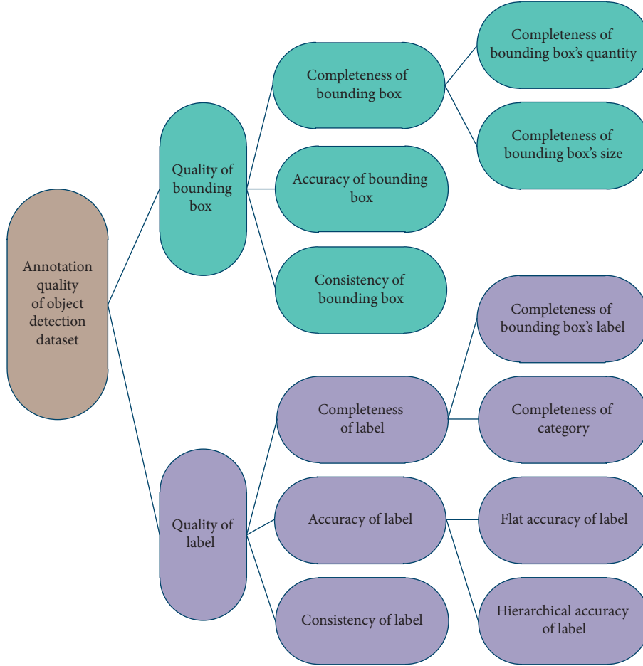
FIGURE 1: Annotation quality evaluation framework.
