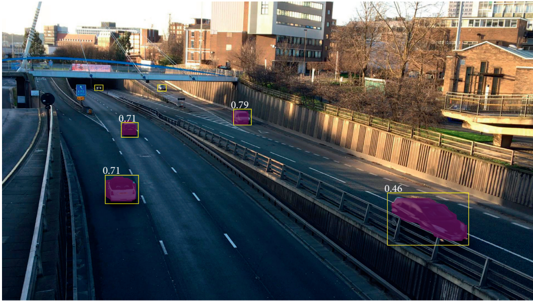
FIGURE 4: Accuracy of the bounding box in an image (note that two small objects are missed by the image instance segmentation algorithm.).
