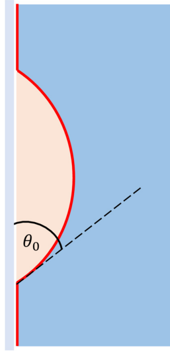
Fig. 3. In field theory a drop on the wall corresponds to the unbinding and recombination of a wall-interface bound state. The contact angle \theta_0 vanishes at the unbinding transition.
