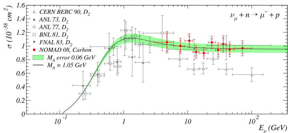
Fig. 18 Comparison of NOMAD \langle\sigma_{\text{qel}}\rangle_{\nu_\mu} measurements with previous \nu_\mu D experimental data (ANL 73 (Argonne 12-foot BC) [2], ANL 77 [3], BNL 81 (Brookhaven 7-foot BC) [6], FNAL 83 (FermiLab 15-foot BC) [9], BEBC 90 (CERN, Big European Bubble Chamber) [18]; corrections for nuclear effects have been made by the
