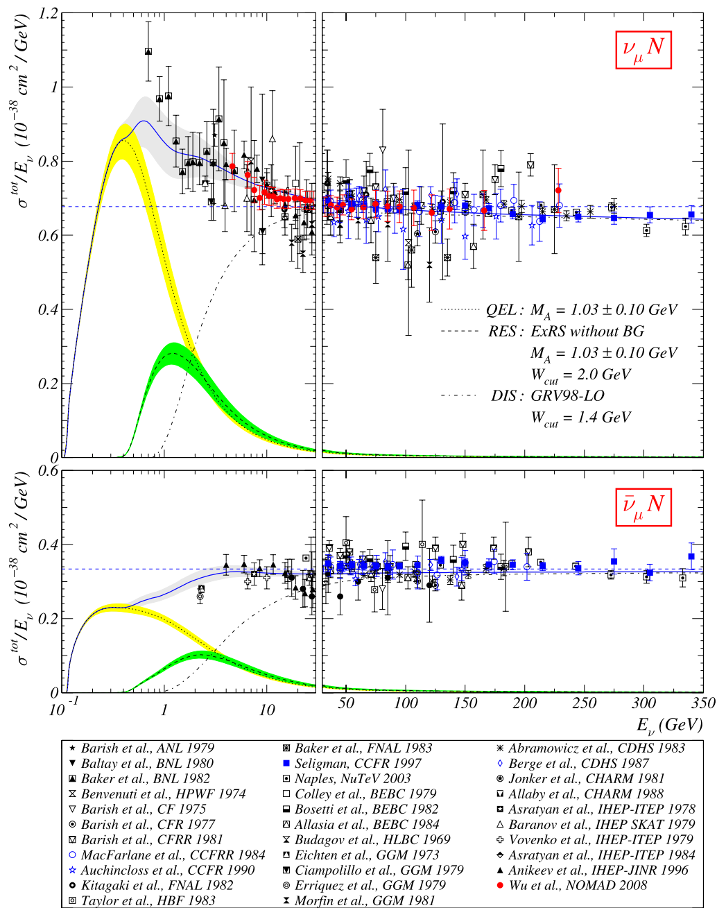
Fig. 5 Slopes of the total \nu_{\mu} and \bar{\nu}_{\mu} CC scattering cross sections off an isoscalar nucleon. Experimental data come from [65] and from [78] for the NOMAD points. The smooth curves show the QEL, RES, and DIS contributions and their sums calculated as described in Sect. 4.6. RES and DIS are used in this analysis to subtract background from experimental data (see (11)). The axial mass M_A , which enters both QEL and RES, is given the value used in
