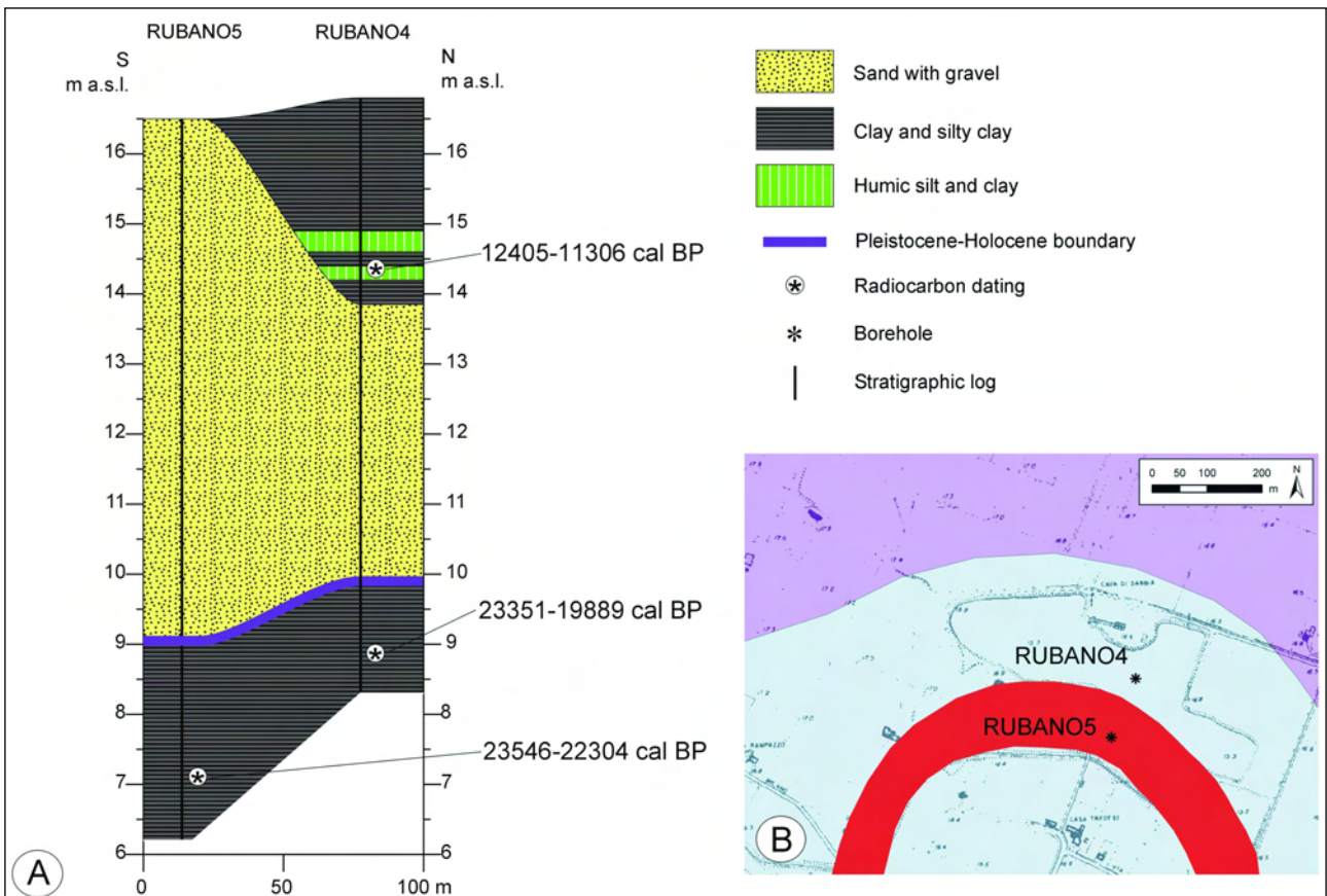
Fig. 6 - Rubano cross section (A) and location map (B) (modified from CASTIGLIONI et al. , 1987).
