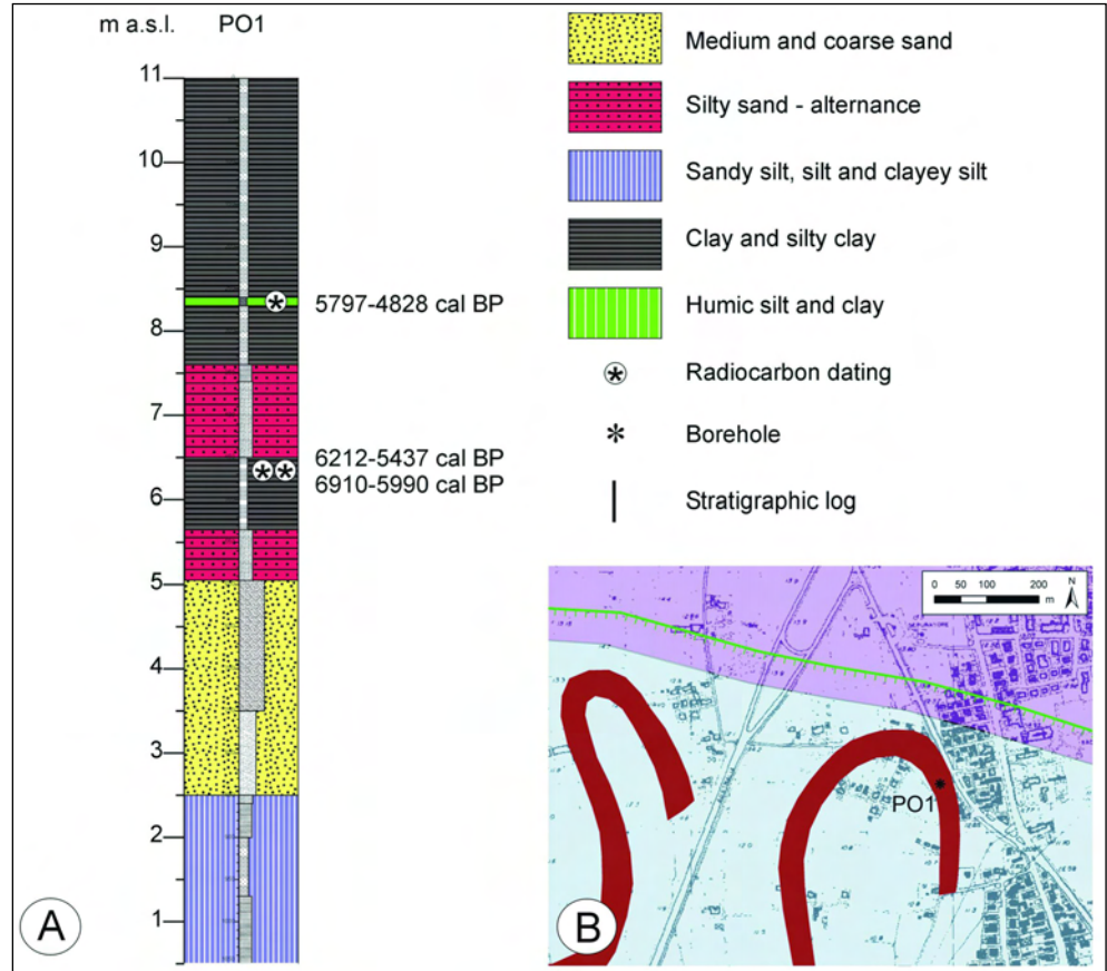
Fig. 5 - Stratigraphic log of PO1 borehole in via Po street in Padua (A) and location map (B) (modified from CASTIGLIONI et al. , 1987).
