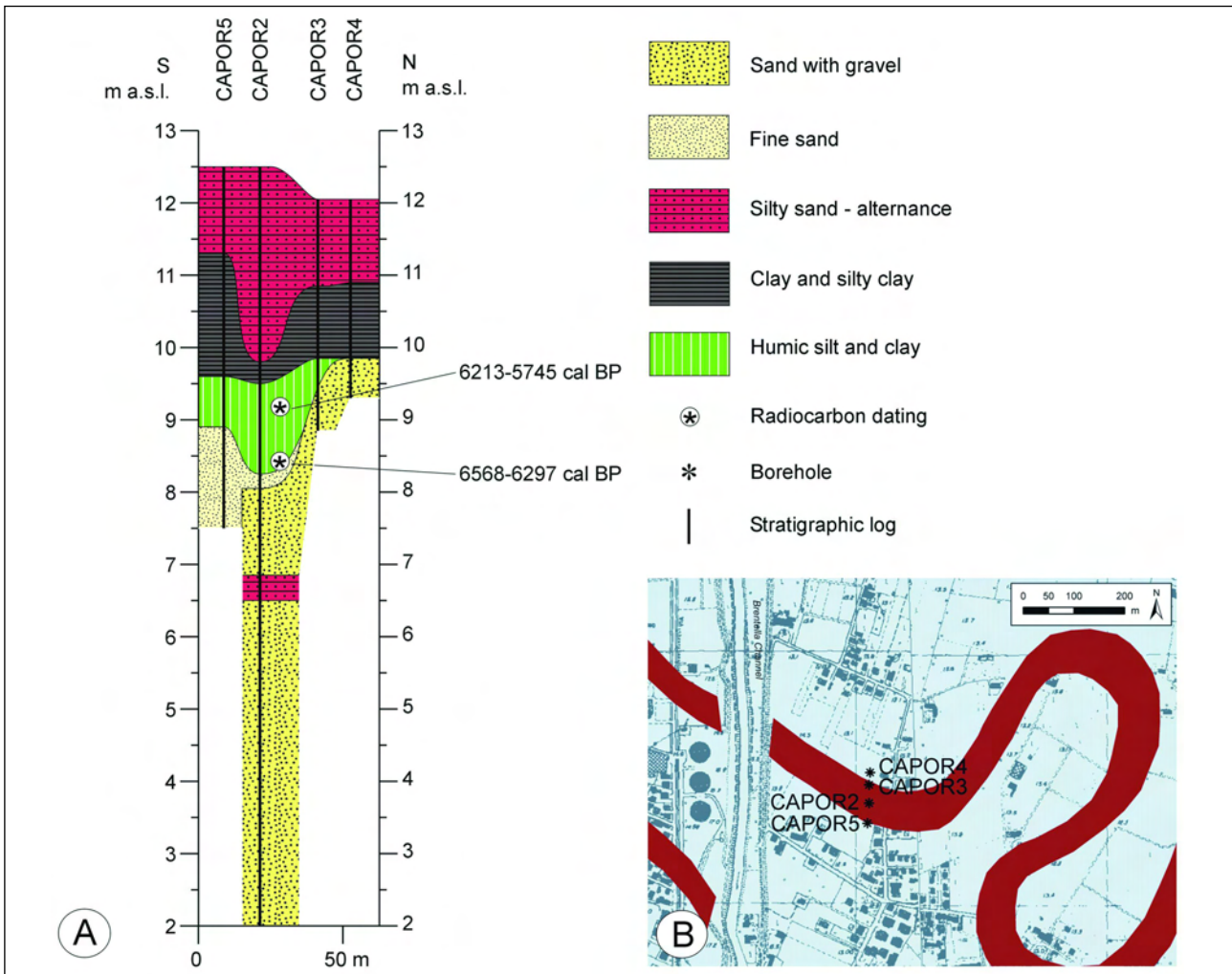
Fig. 4 – Via Caporello cross sections (A) and location map (B) (modified from CASTIGLIONI et al. , 1987).
