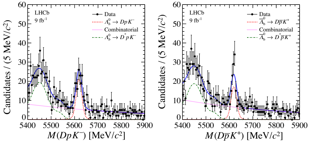
FIG. 3. Distributions of the invariant mass for (left) \Lambda_b^0 \rightarrow [K^+ \pi^-]_D p K^- and (right) \bar{\Lambda}_b^0 \rightarrow [K^- \pi^+]_D \bar{p} K^+ candidates in the full phase space (black points), corresponding to separation of the suppressed decay sample by \Lambda_b^0 flavour. The fit, as described in the text, is indicated by the solid blue line, and individual components are indicated.
