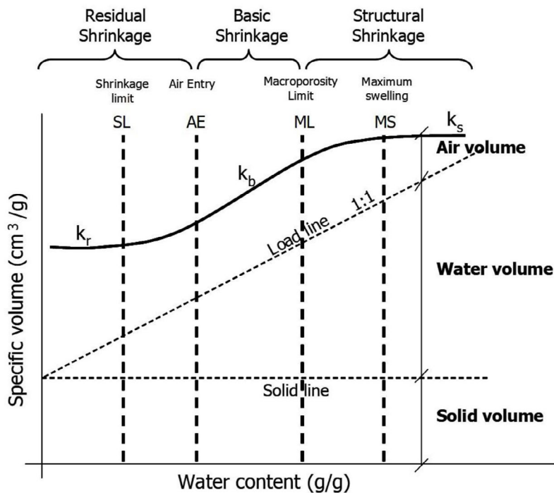
Figure 1. Theoretical shrinkage curve (ShC) of Specific Volume as a function of Soil Water Content, where volumes of solid, liquid and gas components are defined. Transition points of maximum swelling (MS), of macroporosity limit (ML), air entry (AE) and shrinkage limit (SL) are identified. Shrinkage phases: structural ( k_s ), basic ( k_b ) and residual ( k_r ) shrinkage slopes are shown (adapted from Braudeau et al. , 1999).
