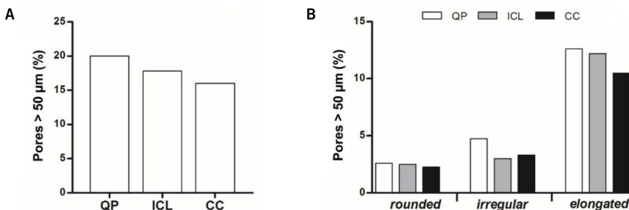
Figure 4. Porosity higher than 50 μm (Pores>50 μm) (a); and pore shape (rounded, irregular, elongated) (b) for managements evaluated: quasi-pristine (QP), integrated crop livestock (ICL) and continuous cropping (CC) in the Argiudoll.
