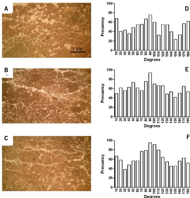
Figure 3. Thin sections and pore-angle frequency distribution of quasi pristine (A, D), integrated crop/livestock (B, E) and continuous cropping (C, F); for the Argiudoll.
