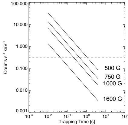
Fig. 6. Expected RHESSI count rates at 250 keV as a function of the emitting electron trapping time for different magnetic field strengths and view angle equal to 84^\circ . Each solid line represents a different solution determined by a different magnetic field. The dashed horizontal line represents the measured background count rate at 250 keV.
