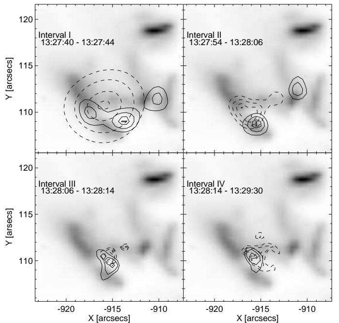
Fig. 5. RHESSI emitting regions of 50 – 100 keV (solid contours) and of 12 - 20 keV (dashed contours) for different time intervals superimposed on a negative 195 \text{ \AA} image taken by TRACE at 1327:31 UT. Contour levels are: 50, 70, 90, and 99% of the image maximum.
