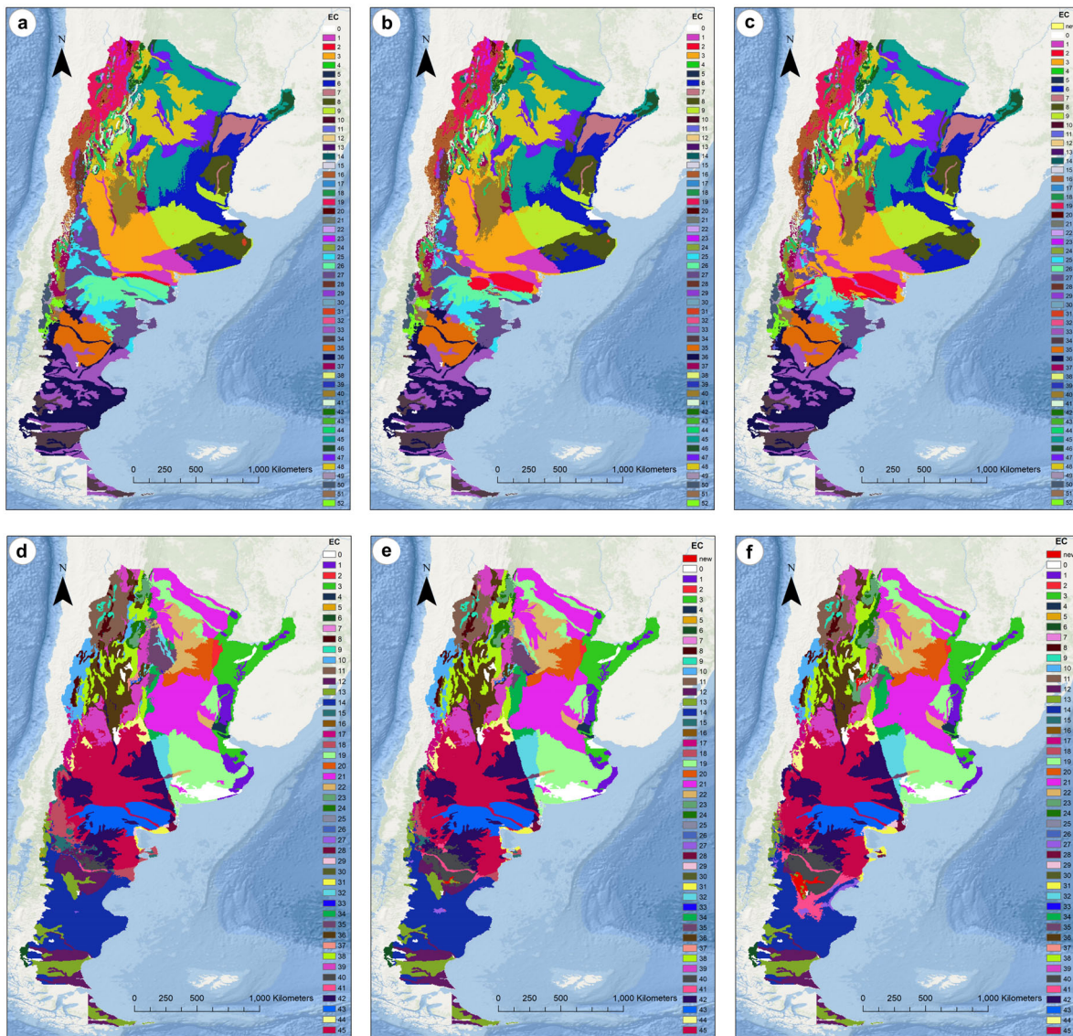
Fig. 3. Ecogeographical land characterization maps generated for Trichloris crinita with ecogeographical data from (a) present, (b) RCP 4.5 scenario for 2050, and (c) RCP 8.5 scenario for 2070, and for Trichloris pluriflora with ecogeographical data from (d) present, (e) RCP 4.5 scenario for 2050, and (f) RCP scenario 8.5 for 2070.
