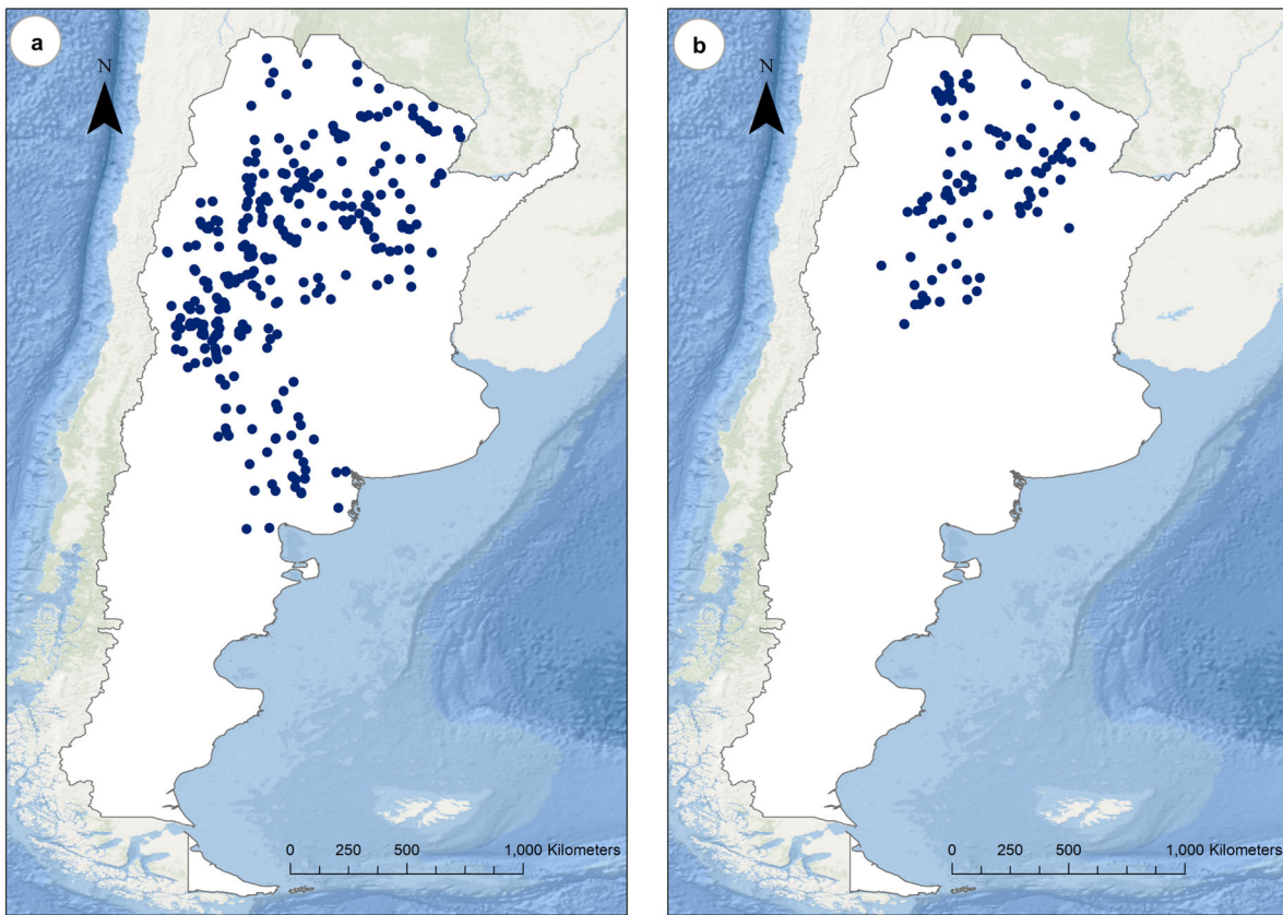
Fig. 1. Species distribution maps: (a) occurrence dataset of Trichloris crinita and (b) occurrence dataset of Trichloris pluriflora .
