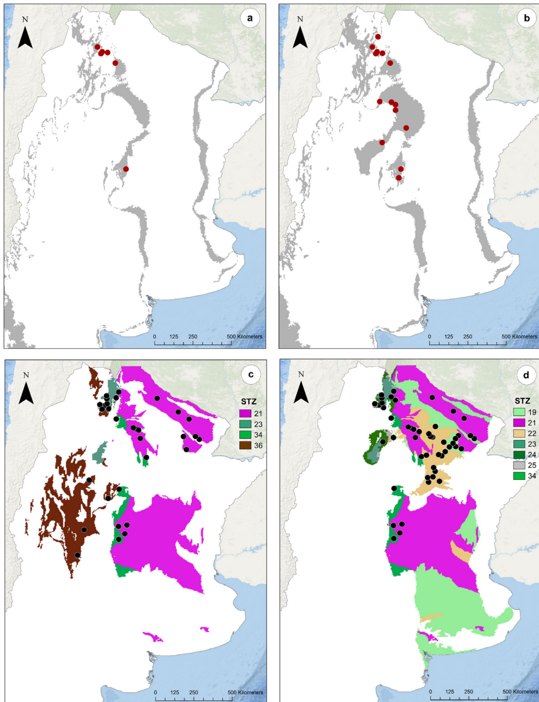
Fig. 6. Climate change impact on Trichloris pluriflora distribution. Changing seed transfer zones (STZs; gray zones) and threatened populations—potential beneficiary populations—(red points) for (a) RCP 4.5 scenario for 2050 and (b) RCP 8.5 scenario for 2070. Spatiotemporal STZs and potential seed source populations (black points) for (c) RCP 4.5 scenario for 2050 and (d) RCP 8.5 scenario for 2070.
