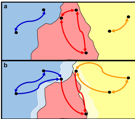
Fig. 2. Germplasm flow between populations (black points) according to seed transfer zone (STZ) structure. The arrows indicate the potential germplasm flow within STZs: (a) potential germplasm flow under present conditions (1950–2000) among populations occurring in three different STZs (solid blue, red, and yellow areas), and (b) potential germplasm flow across spatiotemporal STZs under a climate change scenario. Dashed blue and yellow areas illustrate areas changing from red to blue and yellow STZs, respectively, due to climate change. The tail of the arrows indicates present seed sources that can be used to reinforce future beneficiary populations (head of arrows).
