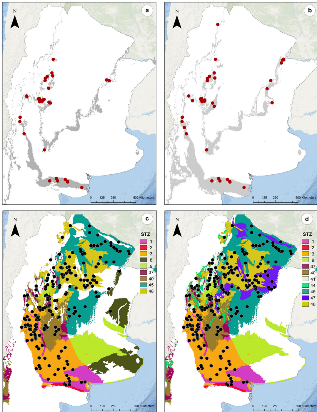
Fig. 5. Climate change impact on distribution of Trichloris crinita . Changes in seed transfer zones (STZs; gray zones) and threatened populations—potential beneficiary populations—red points) for (a) RCP 4.5 scenario for 2050 and (b) RCP 8.5 scenario for 2070. Spatiotemporal STZs and potential seed source populations (black points) for (c) RCP 4.5 scenario for 2050 and (d) RCP 8.5 scenario for 2070.
