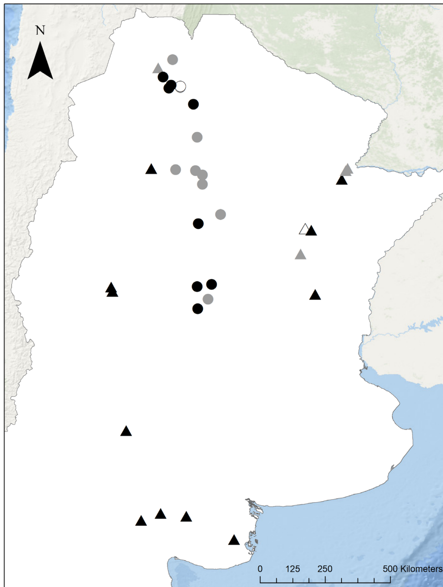
Fig. 7. Final target populations for an optimized collecting design for Trichloris crinita (triangles) and Trichloris pluriflora (circles). Solid black symbols represent prioritized populations in both future scenarios (RCP 4.5/2050 and RCP 8.5/2070), empty symbols show populations only prioritized for RCP 4.5 scenario, and solid gray symbols represent populations prioritized only for RCP 8.5 scenario.
