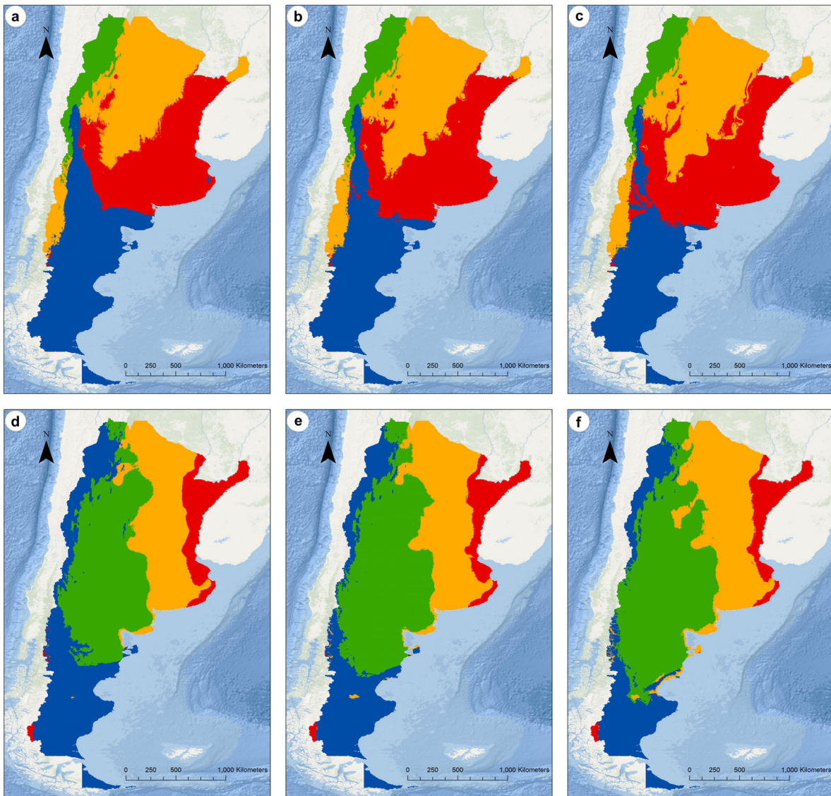
Fig. 4. Bioclimatic groups derived from combination of bioclimatic variables, used to generate ecogeographical land characterization maps for Trichloris crinita : (a) present, (b) RCP 4.5 scenario for 2050, and (c) RCP 8.5 scenario for 2070, and for Trichloris pluriflora : (d) present, (e) RCP scenario 4.5 for 2050, and (f) RCP 8.5 scenario for 2070.
