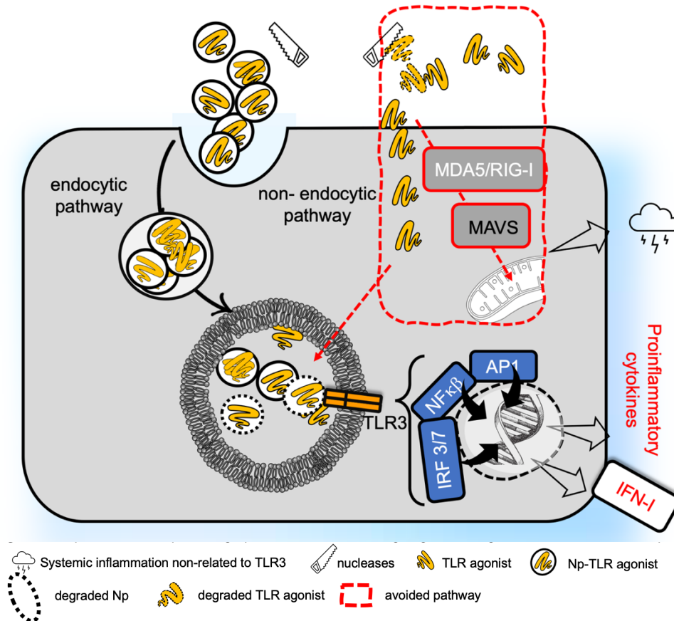
Figure 3. Simplified scheme representing Np-mediated endosomal targeting of TLR3-agonist and avoidance of MAV pathway.
