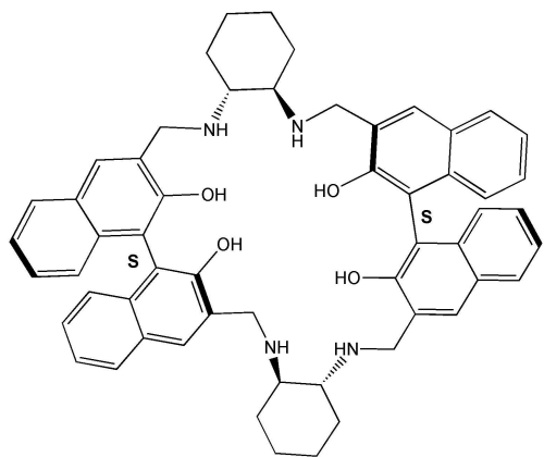
Figure 3. Molecular structure of DACH-based (S) isomer of the bis-binaphthyl macrocycles discussed in Ref. [13].
