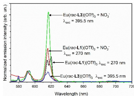
Figure 19. Evolution of the Eu(III) luminescence emission spectra upon addition of the nitrate anion, for complexes Eu( rac -L1)(OTf) 3 and Eu( rac -L3)(OTf) 3 . [Eu( rac -L1)(OTf) 3 ] = [Eu( rac -L3)(OTf) 3 ] = 1 mmol dm -3 ; [NO 3 - ] = 4 mmol dm -3 . OTf = CF 3 SO 3 . Adapted from Ref. [81] with permission (2015) from the Royal Society of Chemistry.
