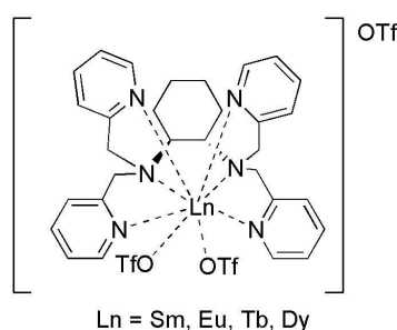
Figure 6. Ln(III) complexes of the ligand (R,R) or (S,S)-tpdac discussed in the paper by G. Ung and co-authors. [55]
