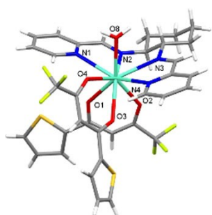
Figure 21. Crystal structure of [EuL1(tta) 2 (H 2 O)] CF 3 SO 3 . Triflate anion is omitted for sake of clarity. Adapted with permission from Ref. [65]. Copyright (2018) American Chemical Society.
