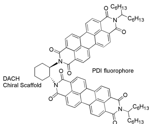
Figure 4. Chemical structure of the molecule discussed in Ref. [15].
