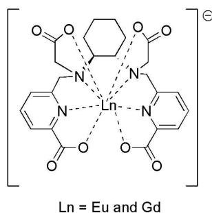
Figure 7. Ln(III) complexes of the ligand (R,R) or (S,S)-cddadpa discussed in the paper by G. Tircsó and co-authors. [57]
