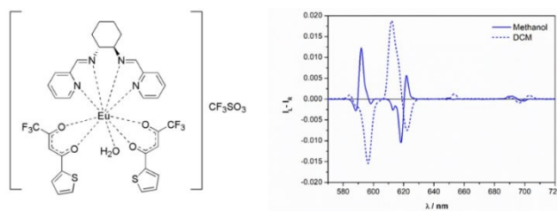
Figure 22. Nearly opposite CPL signature of the (R,R)-[EuL1(tta) 2 (H 2 O)]CF 3 SO 3 complex when dissolved in two different solvents such as methanol and dichloromethane. Adapted from Ref. [91] with permission, available at https://pubs.acs.org/doi/10.1021/acs.inorgchem.0c00280 ; further permissions related to the material excerpted should be directed to the ACS.
