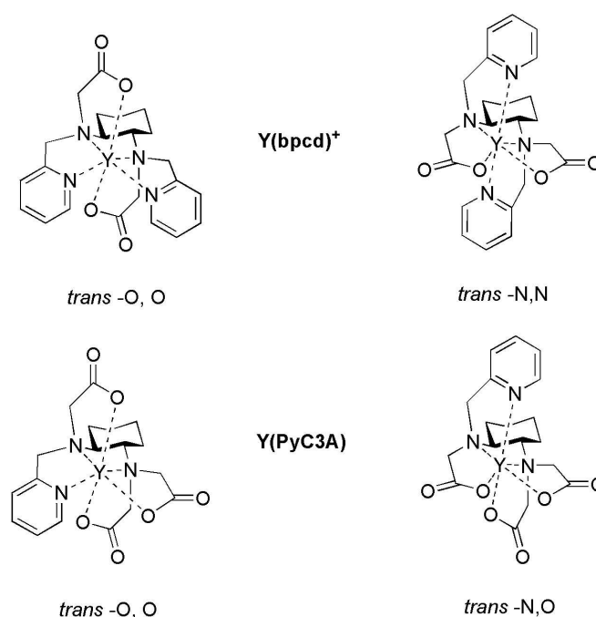
Figure 11. Possible stereoisomeric complexes found by DFT calculations. In the case of cationic complexes with \text{bpcd}^{2-} , \text{bQcd}^{2-} and \text{isobQcd}^{2-} ligands, trans-O,O and trans-N,N species are observed. In the case of neutral complexes with \text{PyC3A}^{3-} , \text{QC3A}^{3-} and \text{isoQC3A}^{3-} ligands, trans-O,O and trans-N,O species are observed. Only the representative pyridine-based complexes are depicted in this figure. Water molecules bound to the metal ion are omitted for sake of clarity.
