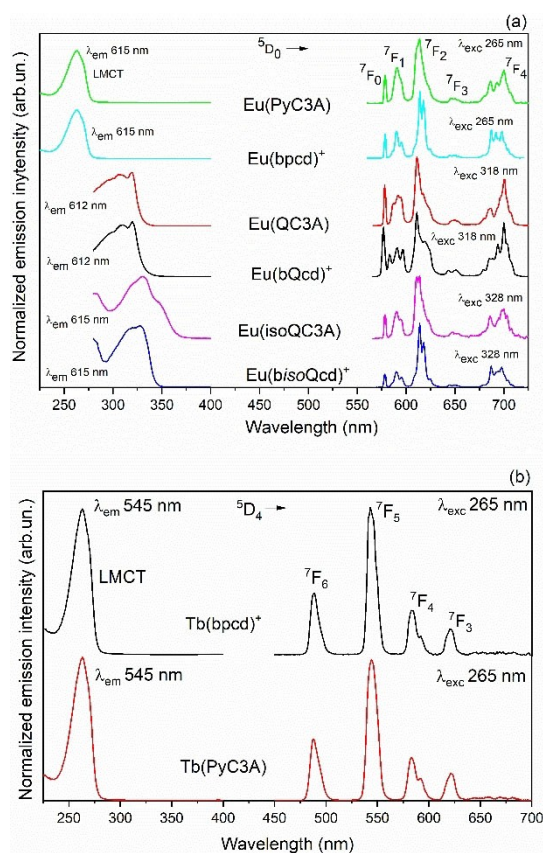
Figure 12. (a) Excitation and emission spectra of Eu(III) complexes depicted in Figure 9. (b) Excitation and emission spectra of Tb(III) complexes of the ligands bpcd 2- and PyC3A 3- .
