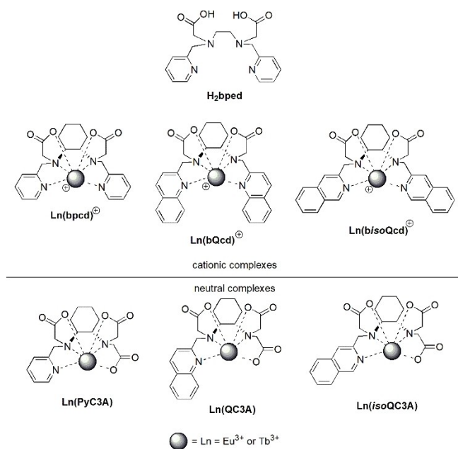
Figure 9. Chemical structure of H 2 bped ligand and of the Eu(III) and Tb(III) complexes discussed in section 2.4. bpced 2- = N,N'-bis(2-pyridylmethyl)-trans-1,2-diaminocyclohexaneN,N'-diacetate; bQcd 2- = N,N'-bis(2-quinolinmethyl)-trans-1,2-diaminocyclohexane N,N'-diacetate; bisoQcd 2- = N,N'-bis(2-isoquinolinmethyl)-trans-1,2-diaminocyclohexane N,N'-diacetate; PyC3A 3- = N-picolyl-N,N'-trans-1,2-cyclohexylenediaminetriacetate; QC3A 3- = N-quinolyl-N,N'-trans-1,2-cyclohexylenediaminetriacetate; isoQC3A 3- = N-isoquinolyl N,N'-trans-1,2-cyclohexylenediaminetriacetate.
