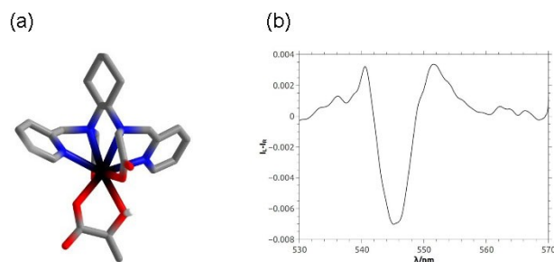
Figure 14. (a) Minimum energy structures of the [\text{Y}(\text{S,S-bpcd})\text{L-lactate}] complex in the case of trans -Npy, Npy isomer. (b) CPL spectrum of [\text{Tb}(\text{rac-bpcd})^+] (5 mM) in a commercial Ringer's lactate solution, upon excitation at 265 nm. Adapted from Ref. [79] with permission (2018) from the Centre National de la Recherche Scientifique (CNRS) and the Royal Society of Chemistry
