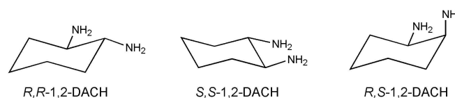
Figure 1. Chemical structure of DACH – trans -1,2-diaminocyclohexane (both R,R and S,S -1,2-DACH enantiomers) and DACH – cis -1,2-diaminocyclohexane ( meso achiral isomer).
