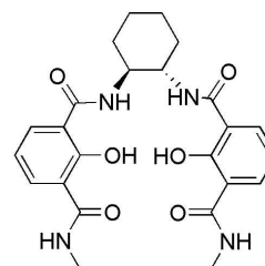
Figure 8. CyLI-IAM as ligand of Tb(III). [58]
