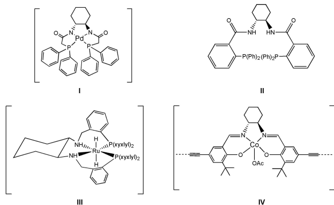
Figure 2. Chemical structure of the DACH-based catalytic complexes discussed in the text.
