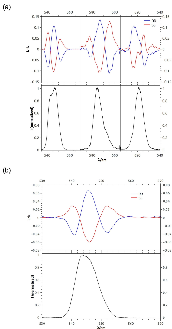
Figure 13. Normalized CPL spectra (top) and total emission (bottom) of the two enantiomers of \text{Tb}(\text{bpcd})^+ in \text{CD}_3\text{OD} (a) and water (b). The curves in each panel are normalized on the maximum of the corresponding total emission band. Adapted with permission from Ref. [61]. Copyright (2017) American Chemical Society.
