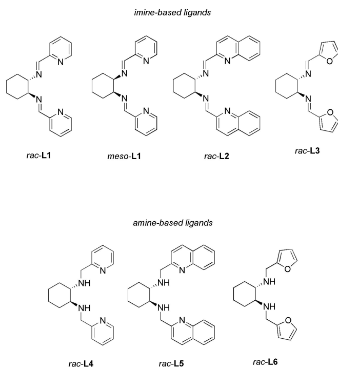
Figure 18. Structure of the molecules used as tetradentate ligands for Ln(III) discussed in this section.
