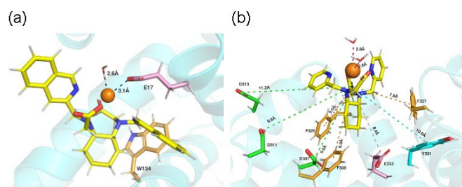
Figure 16. Snapshot of the interaction site of BSA with the [Y( biso Qcd)(H 2 O)] + (a) and [Eu(bpccd)(H 2 O) 2 ] + (b) complexes. Adapted from Ref. [53] with permission, available at https://pubs.acs.org/doi/10.1021/acs.inorgchem.0c01663 ; further permissions related to the material excerpted should be directed to the ACS.
