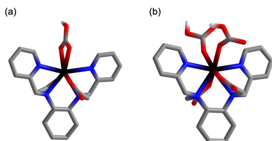
Figure 15. Minimum energy structures of (a) [Y( trans -O,O-bpccd)(HCO 3 ) 2 ] + and (b) [Y( trans -O,O-bpccd)(HCO 3 ) 2 ] - which present the unusual bis -hydrogen carbonate coordination mode. Adapted from Ref. [63] with permission (2019) from the Royal Society of Chemistry
