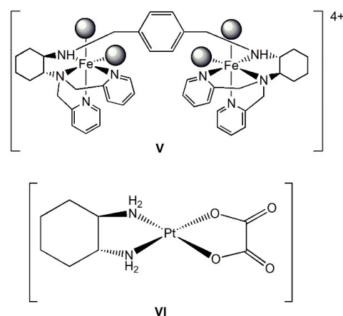
Figure 5. Chemical structure of p-R-BDC derivative (compound V) and oxaliplatin (compound VI). Grey spheres represent solvent molecules.
