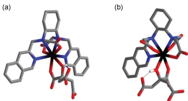
Figure 17. Minimum energy structures of (a) [Y(\text{bisoQcd})\text{cit}]^{2-} and (b) [Y(\text{isoQC3A})\text{cit}]^{3-} adducts; cit = citrate. trans -O,O isomers are considered.
