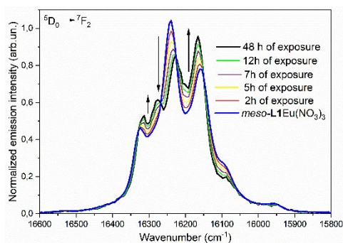
Figure 20. Evolution over the time of the Eu(III) ^5D_0 \rightarrow ^7F_2 luminescence emission band of the [Eu( meso -L1)(NO 3 ) 3 ] complex upon exposure to acetonitrile vapor. Excitation was at 273 nm. Adapted with permission from Ref. [90]. Copyright (2021) Elsevier.
