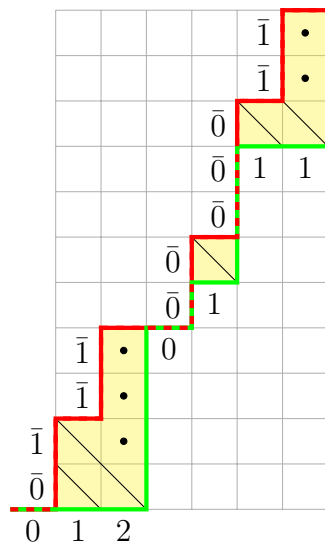
Figure 3: A 6 \times 11 reduced polyomino. Its area word is 0\bar{0}1\bar{1}2\bar{1}\bar{1}1\bar{0}\bar{0}\bar{0}\bar{0}\bar{0}\bar{0}1\bar{1}\bar{1}\bar{1} .
