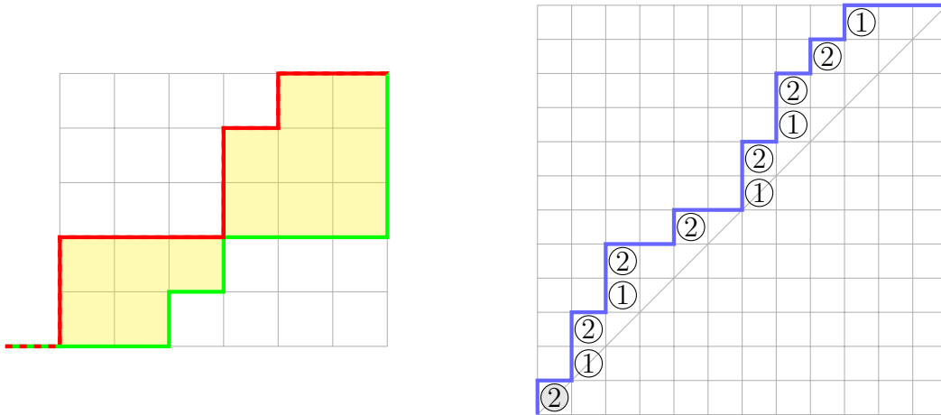
Figure 6: A reduced polyomino (left) with area word 00\bar{1}\bar{1}2100\bar{1}\bar{1}22\bar{2} and its corresponding two car parking function (right).
