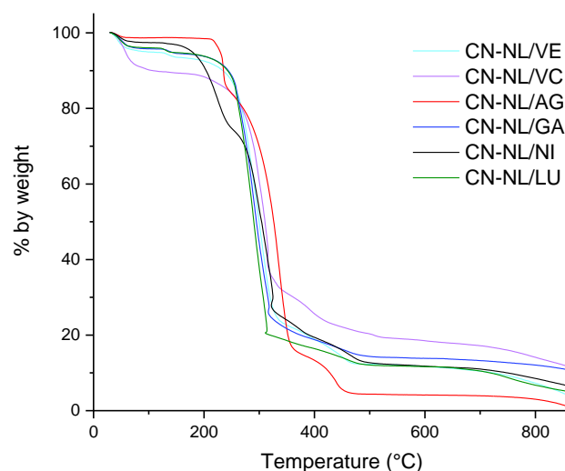
Figure 8. TGA thermograms of spray-dried CN-NL/M complexes.
