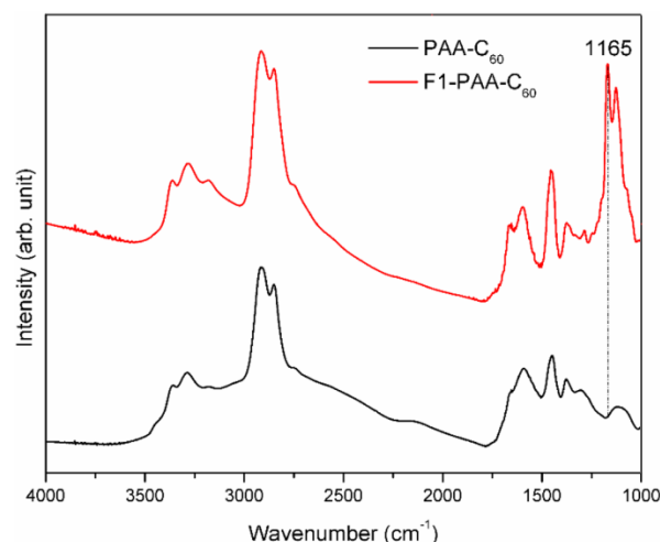
Figure 2. FTIR spectra of PAA-C 60 and F1-PAA-C 60 . Prior to analysis the materials were vacuum-dried at 90 °C. Full peak assignments are given in Figure S3 (see SI).
