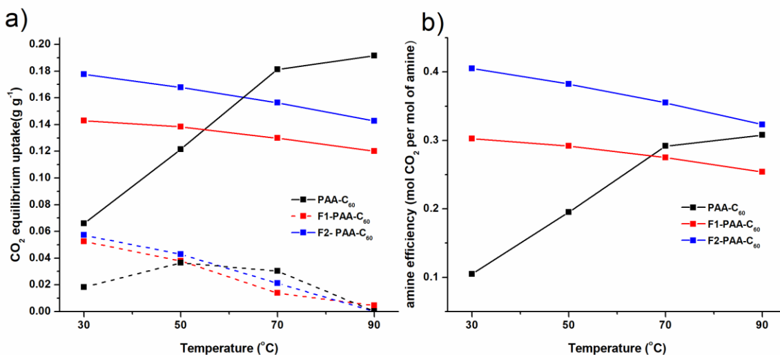
Figure 3. a) CO_2 uptake vs temperature for PAA- C_{60} (black), F1-PAA- C_{60} (red) and F2-PAA- C_{60} (blue) in 100% CO_2 (solid lines) or 400 ppm CO_2 in N_2 (dashed lines); b) amine efficiency in 100% CO_2 as a function of temperature, PAA- C_{60} (black), F1-PAA- C_{60} (red) and F2-PAA- C_{60} (blue).
