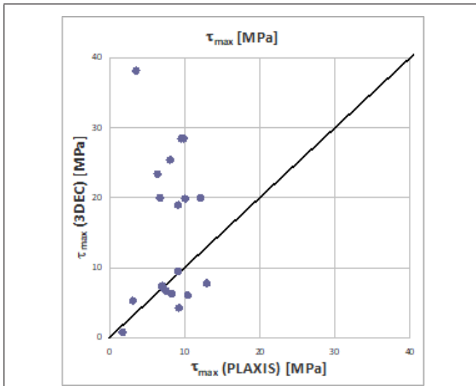
Figure 7: Maximum shear stresses at the monitoring points.
