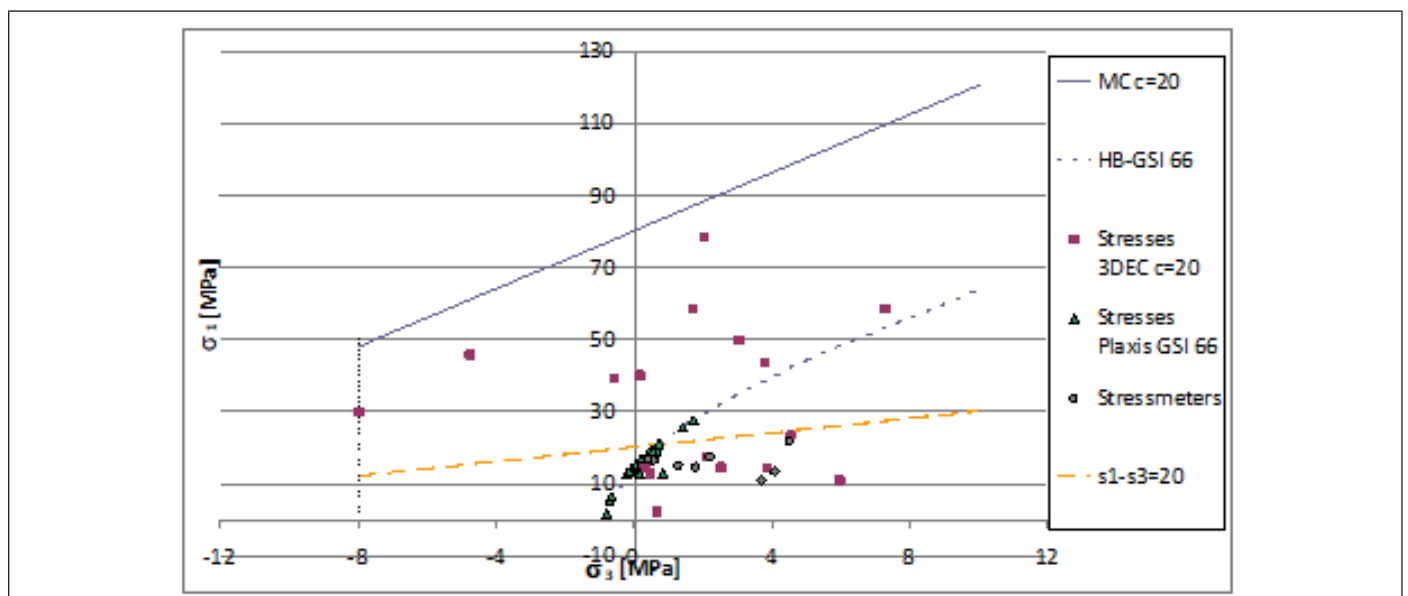
Figure 9: Failure envelopes (Tresca type, MC and HB), in situ principal stress measurements and those inferred from 3DEC and PLAXIS analyses.
