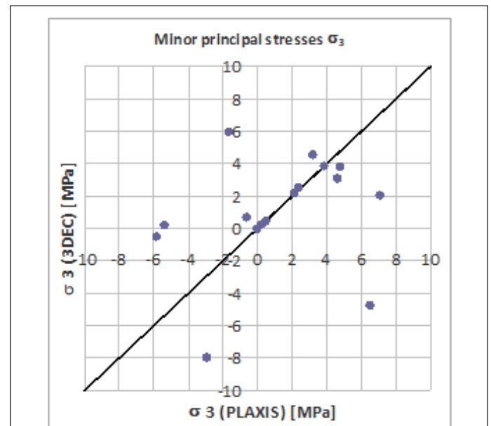
Figure 6: Minor principal stresses at the monitoring points.
