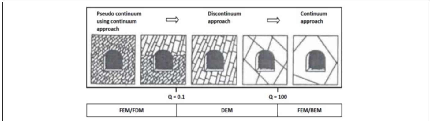
Figure 1: Schematic diagram suggesting the range of application of dis-continuum modeling in relation to Q value ([9] modified by [10]). (for the study case Q is about 7; RMR = 9 \cdot LNQ + 44 )
