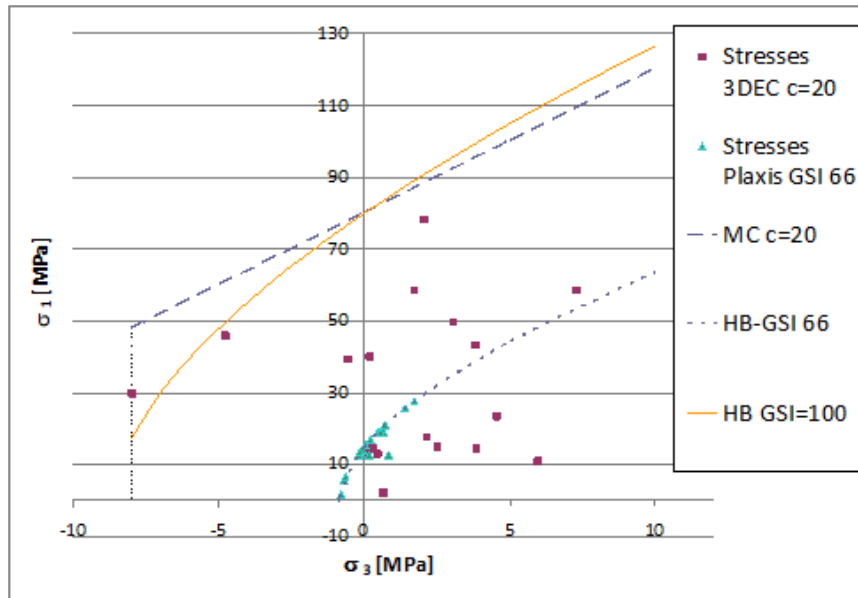
Figure 4: Failure envelopes (MC & HB) in the principal stresses plane and stresses values inferred from PLAXIS & 3DEC analyses.
