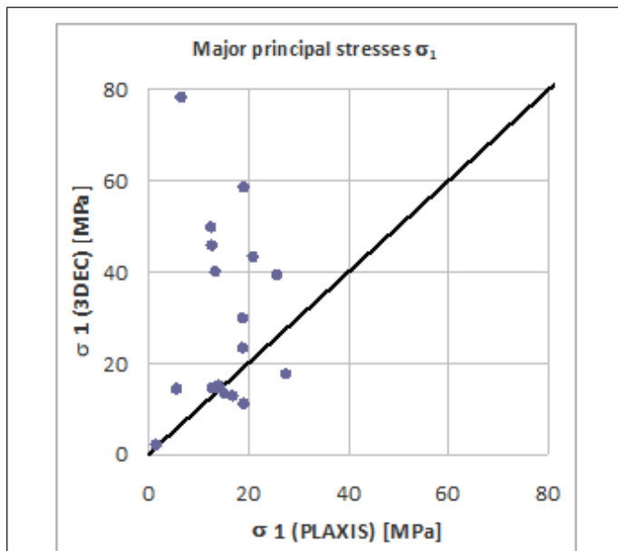
Figure 5: Major principal stresses at the monitoring points.
