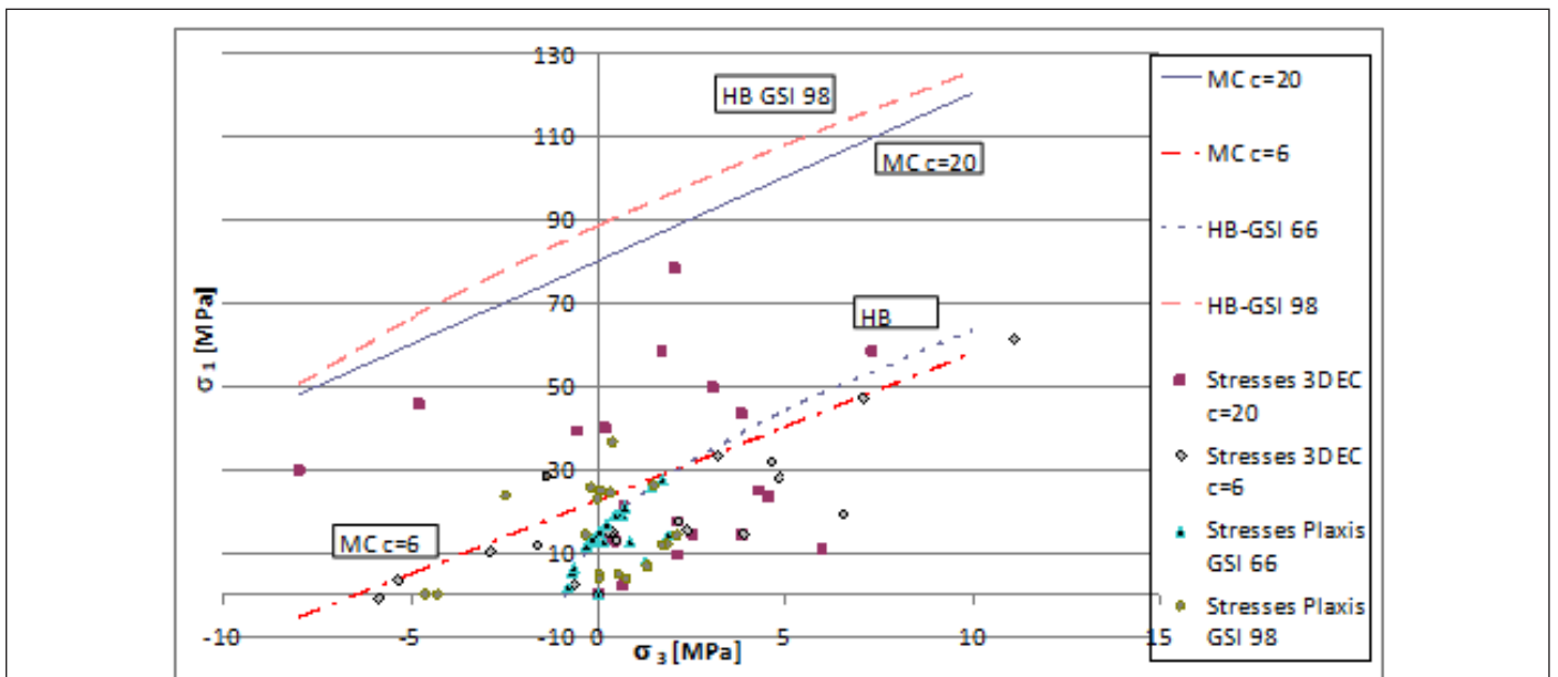
Figure 8: Equivalent failure envelopes (MC & HB) in the principal stress plane and stress values from PLAXIS & 3DEC at the monitoring points.
