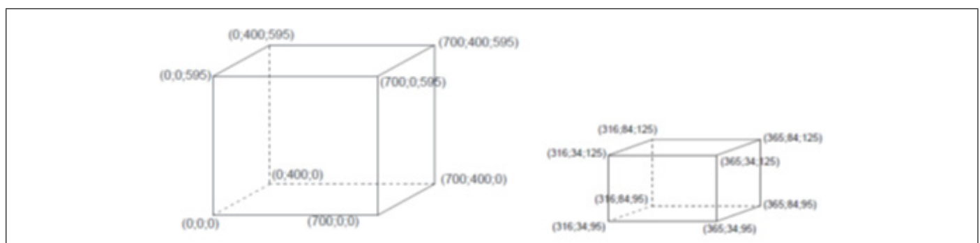
Figure 2: Absolute coordinates (x, y, z) of the block (on the left) and of the internal cavity (on the right).
