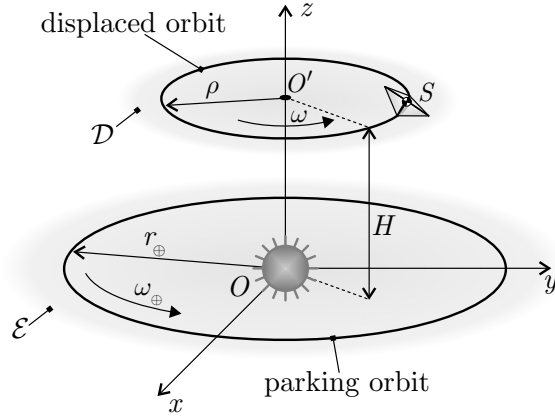
Figure 2: Conceptual scheme of heliocentric circular displaced orbit.
