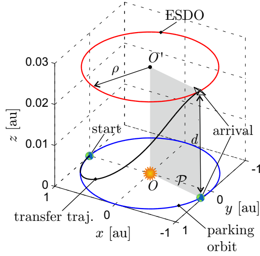
Figure 13: Optimal transfer trajectory towards an ESDO with H = 0.026 au and \rho = 0.985 au.
