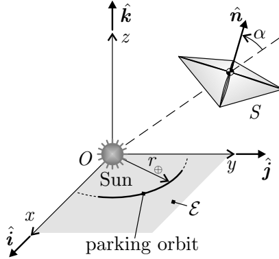
Figure 1: Inertial reference frame \mathcal{T}(O; x, y, z) and sail cone angle \alpha .
