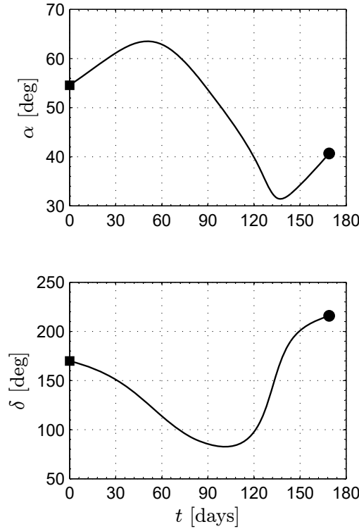
Figure 13: Optimal transfer trajectory towards an ESDO with H = 0.026 au and \rho = 0.985 au.
