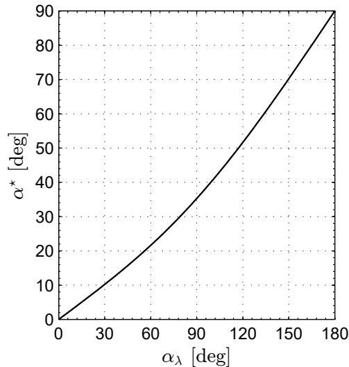
Figure 8: Optimal sail cone angle \alpha^* as a function of the primer vector cone angle \alpha_\lambda .
