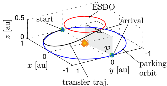
Figure 10: Optimal transfer trajectory towards an ESDO with H = \rho = 0.5 \text{ au} .
