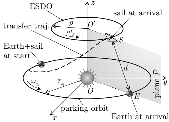
Figure 2: Conceptual scheme of heliocentric circular displaced orbit.
