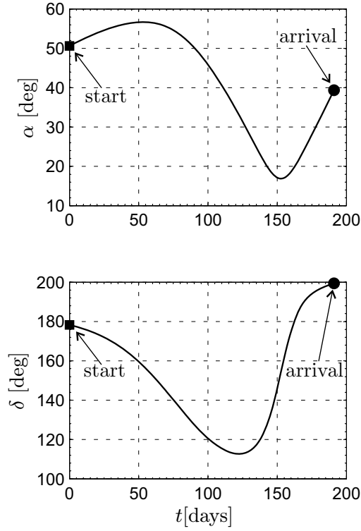
Figure 11: Optimal control law for a transfer towards an ESDO with H = \rho = 0.5 au.
