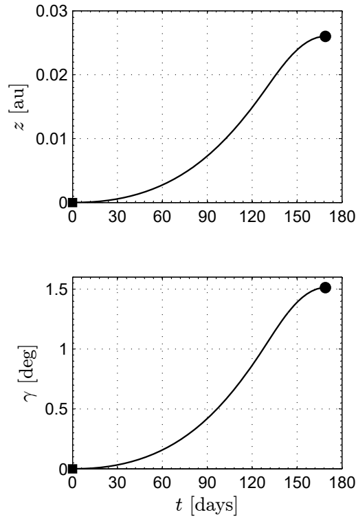
Figure 15: Spacecraft ecliptic displacement and inclination angle for a transfer towards an ESDO with H = 0.026 au and \rho = 0.985 au.
