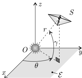
Figure 5: Spherical (heliocentric) reference frame \mathcal{T}_S(O; r, \theta, \gamma) .
