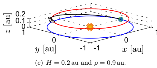
Figure 9: Optimal orbit-to-orbit transfer trajectories for the mission scenarios discussed in Ref. [28] ( T = 1 year).
