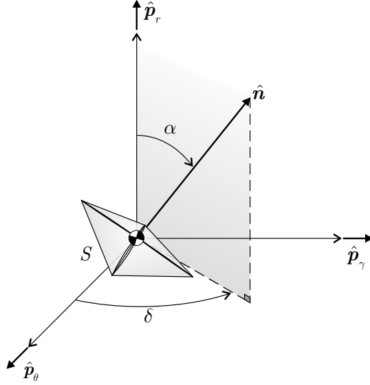
Figure 6: Ideal solar sail thrust vector control angles \{\alpha, \delta\} .
