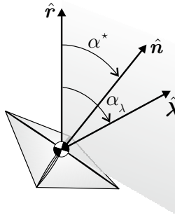
Figure 7: Optimal configuration of \hat{\boldsymbol{\lambda}} , \hat{\boldsymbol{r}} , and \hat{\boldsymbol{n}} .
