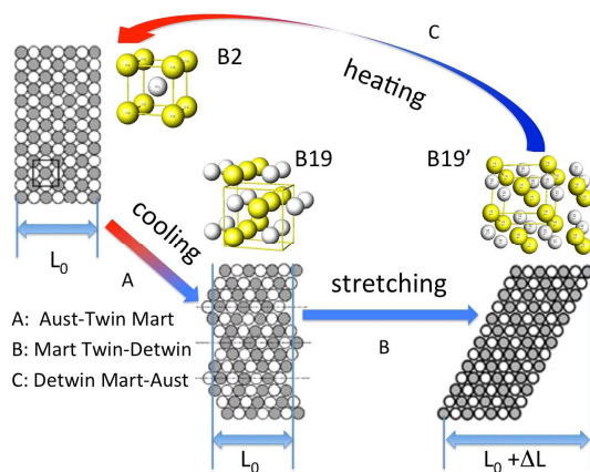
Fig. 2. Thermal and mechanical induced transition in Shape Memory Alloys
