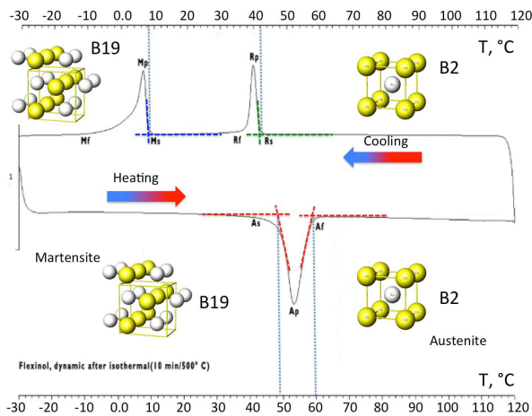
Fig. 3. DSC analysis performed for a specimen of Flexinol wire. Heating segment from -30 to 120°C, cooling segment from 120 to -30°C. Heating and cooling rates 10°C/min
