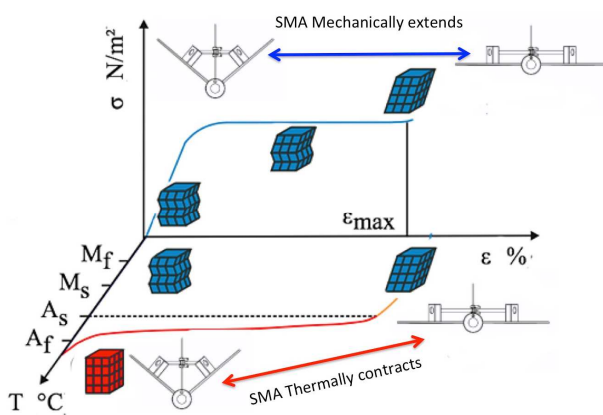
Fig. 6. Thermo-mechanical transformations of SMA adductor and abductor of the biomechanically inspired machine
