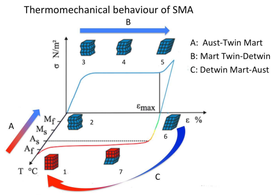
Fig. 1. SST diagram of thermal and mechanical induced transition in Shape Memory Alloys
