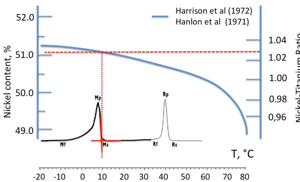
Fig. 4. Detail of DSC characterization of the NiTi alloy composition in the cooling stage
