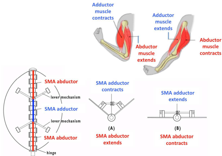
Fig. 5. Biomechanically inspired SMA driven machine
