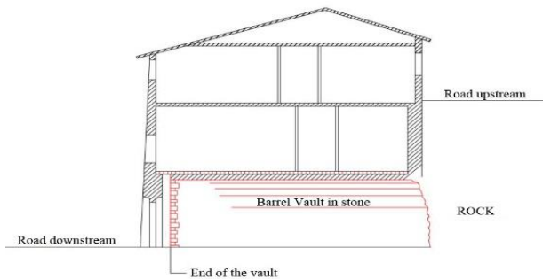
Figure 4. Schematic representation of the typical Structural Unit presents in Campi Alto di Norcia.
