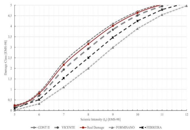
Figure 14. Vulnerability curves for different seismic intensities using the I v methods selected.
