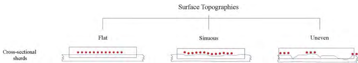
Fig. 5. Red dots indicate the burnishing distribution on flat, sinuous and uneven topographies. (For interpretation of the references to colour in this figure legend, the reader is referred to the web version of this article.)
