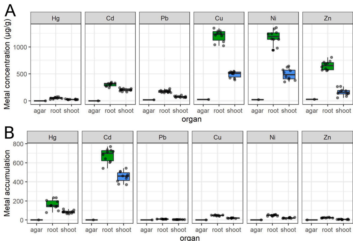
Fig. 1. (A) Metals concentrations in organs and (B) rate of accumulation compared to agar concentration in roots and shoots of Arabidopsis seedlings.
