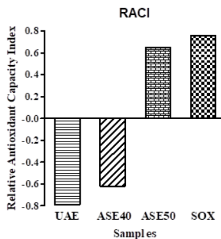
Figure 3. Relative Antioxidant Capacity Index (RACI) values obtained comparing TPC, DPPH, ORAC and BCB results of Aglianico leaf extracts. Samples are extracts obtained by Soxhlet extractive technique (SOX), Accelerated Solvent Extraction at 50 °C (ASE 50) and Ultrasound Assisted Extraction (UAE).
