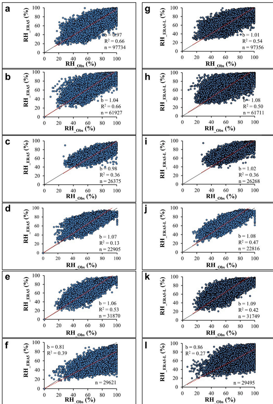
Fig. 5. Daily predicted relative air humidity (RH ERA5 and RH ERA5-L , %) versus observed (RH Obs , %) values at the irrigation districts located in Lombardy (a, g), Emilia-Romagna (b, h); Campania (c, i), Western Sicily (d, j), Eastern Sicily (e, k) and Apulia (f, l) for the period 2008–2020. The black and red lines represent the 1:1 and the linear regression line through the origin, respectively. The terms b, R 2 and n refer to the slope of the regression equation, the coefficient of determination and the number of observations, respectively.
