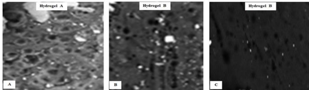
Figure 4. Morphology of Hydrogel A obtained via use of SEM at (A) X500. Morphology of Hydrogel B (B) X1.00k and (C) X2.00k at 10.0KV.
