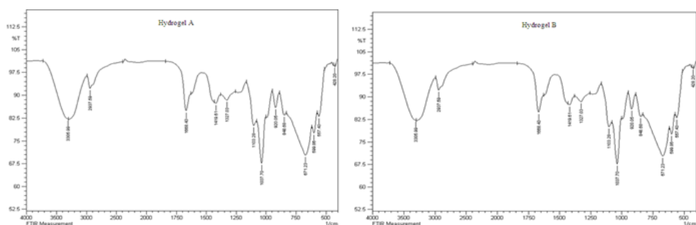
Figure 3. Comparison of FTIR of Hydrogel A and B.
