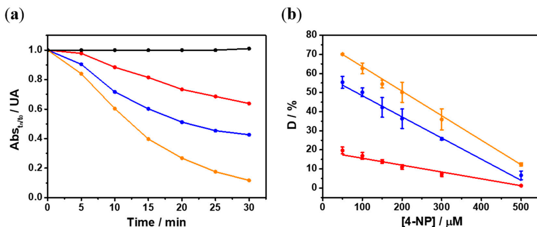
Figure 3. (a) Kinetic curves of 4-NP (100 \mu\text{M} ) reduction at 4-AP in the presence of 0.01 M \text{NaBH}_4 by using the \mu\text{-T@PDA} (black curve), \mu\text{-T@Au} (red curve), \mu\text{-T@Ag} (blue curve), and \mu\text{-T@Au@Ag} (orange curve). (b) Dose–response curves of 4-NP carried out in presence of 0.01 M \text{NaBH}_4 by using the \mu\text{-T@Au} (red curve), \mu\text{-T@Ag} (blue curve), and \mu\text{-T@Au@Ag} .
