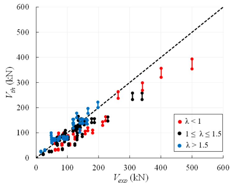
Figure 14. Experimental vs. theoretical results of regular masonry walls provided by Equations (13), (14) and (16) assuming b = 1.5 .
