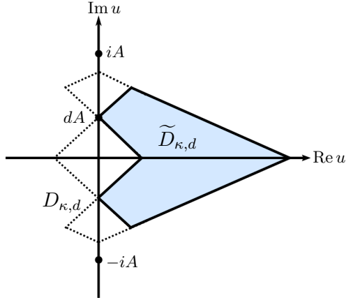
Figure 6: The domain \tilde{D}_{\kappa,d} defined in (3.16).
