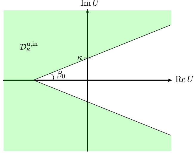
Figure 8: The inner domain \mathcal{D}_\kappa^{\text{u,in}} for the unstable case.
