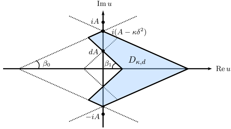
Figure 4: The boomerang domain D_{\kappa, d} defined in (3.7).
