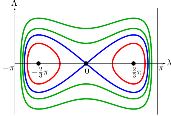
Figure 2: Phase portrait of the system given by Hamiltonian H_p(\lambda, \Lambda) on (2.6). On blue the two separatrices.
