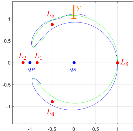
Figure 1: Projection onto the q -plane of the Lagrange points (red) and the unstable (blue) and stable (green) manifolds of L_3 , for \mu = 0.0028 .
