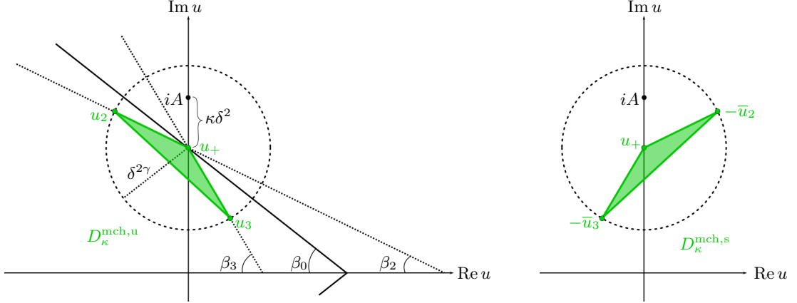
Figure 9: The matching domains D_\kappa^{\text{mch},u} and D_\kappa^{\text{mch},s} in the outer variables.
