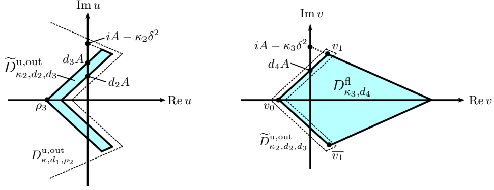
Figure 7: The domain \widetilde{D}_{\kappa_2, d_2, d_3}^{\text{u, out}} given in (3.17) (left) and D_{\kappa_3, d_4}^{\text{fl}} in (3.19) (right).
