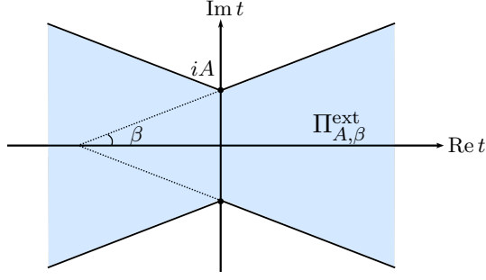
Figure 3: Representation of the domain \Pi_{A,\beta}^{\text{ext}} in (3.2).
