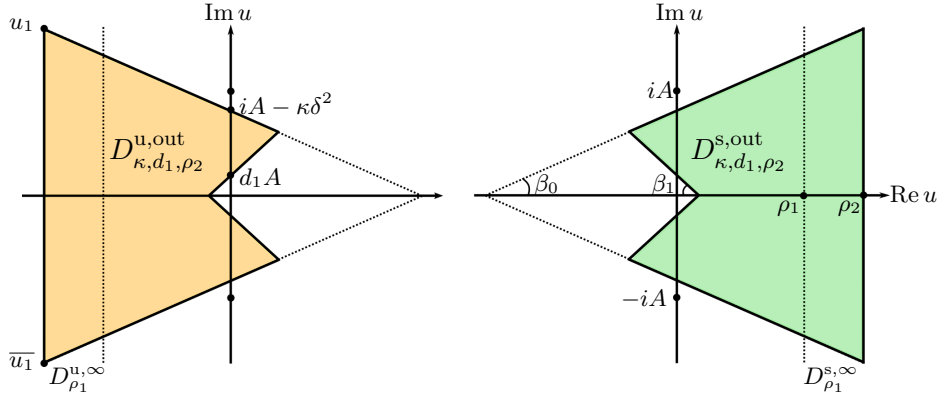
Figure 5: The outer domains D_{\kappa, d_1, \rho_2}^{u, out} and D_{\kappa, d_1, \rho_2}^{s, out} defined in (3.15)
