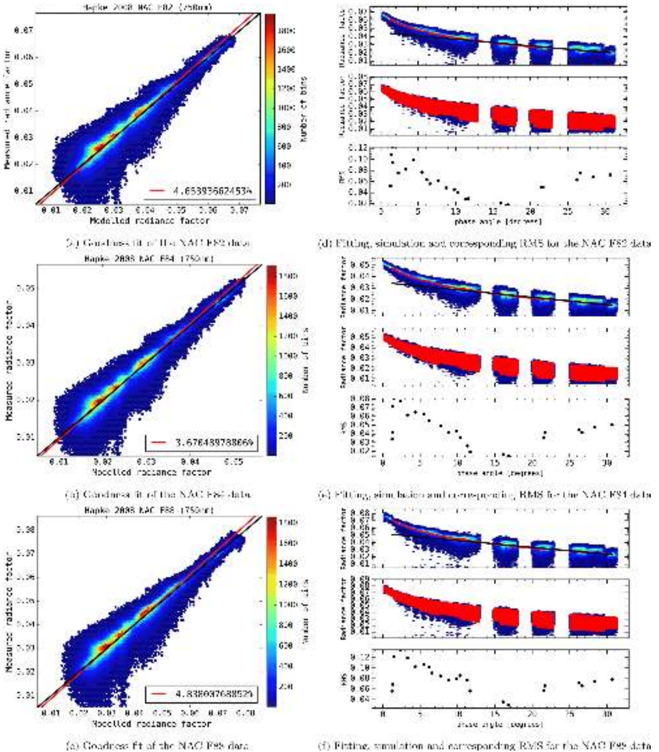
Figure 12. Figures from the Hapke modelling. On the left-hand side, the three figures depicts for all three filters the measured RADF versus the modelled RADF. The black line represent a slope of 1 (i.e. a perfect match). The red line is our best linear fit by taking into account all active cells. On the right-hand side, the three panels of figures present the results of the photometric modelling for each NAC filter. In each figure, the diagram at the top corresponds to the phase function in the corresponding filter with the curve being the best-fitting solution of the photometric modelling. The diagram in the middle presents an overplot of the same phase function with the simulation of the data set using the 3D model and the best-fitting solution. Finally, the diagram at the bottom displays the mean of the rms for each image. In all of these figures, as the measured radiance factor values have been binned, the first and second diagrams show a underplotted density distribution of the active cells.
