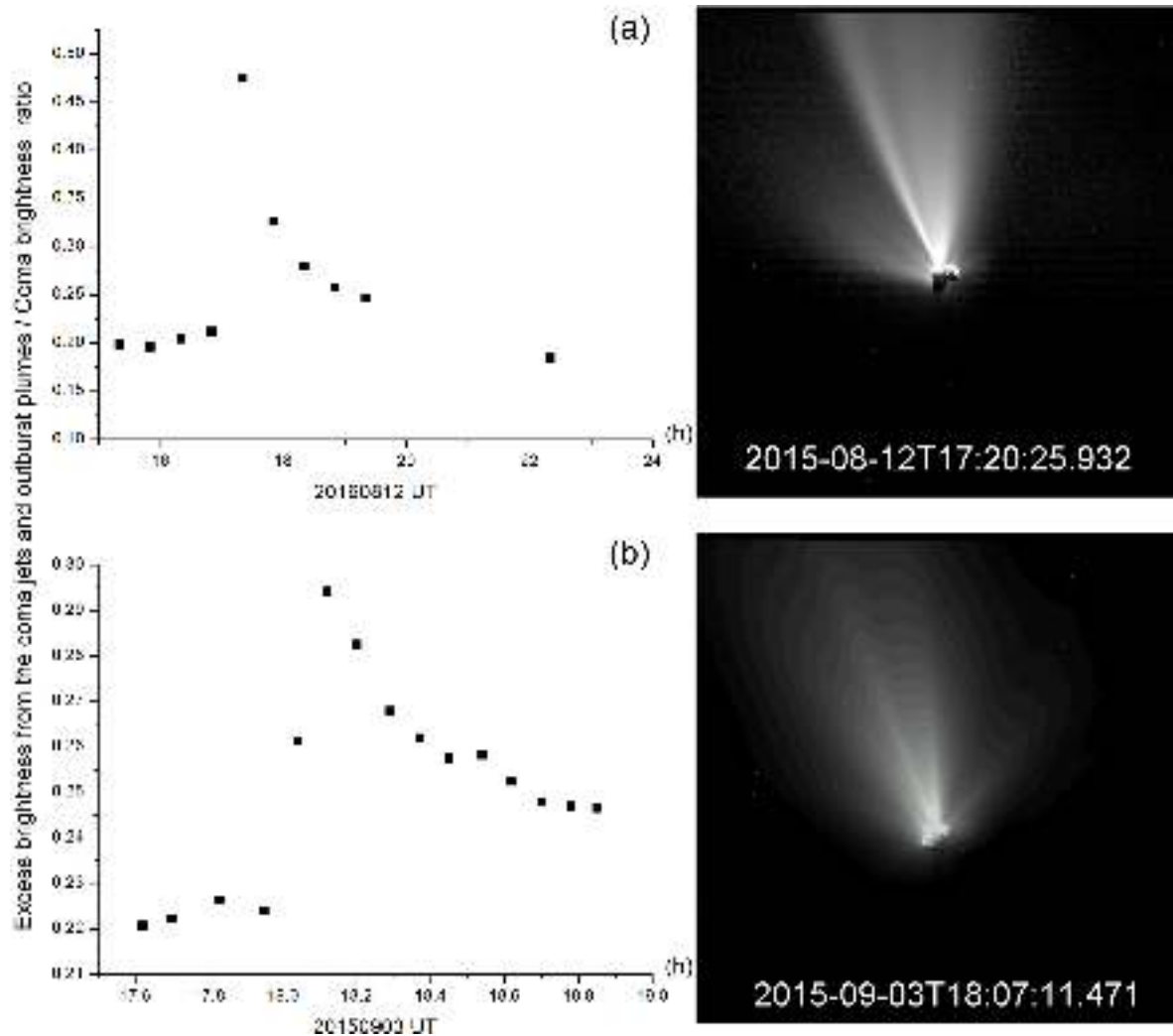
Figure 3. The coma brightness variation estimated from two different sequences: the activity monitoring sequence (top-left panel) and the outburst sequences (bottom-left panel) from the filter UV375 in the WAC. The related outburst images detected at the time of peak value in coma brightness ratio are shown in the right panels. The FOV of these two WAC frames is 67.78 km (a) and 177.65 km (b) and the Sun is towards the top. The maximum excess brightness for the outburst plume is derived from the comparison in between the base that mostly came from the contribution of the coma jets and the peak of the brightness variation.
