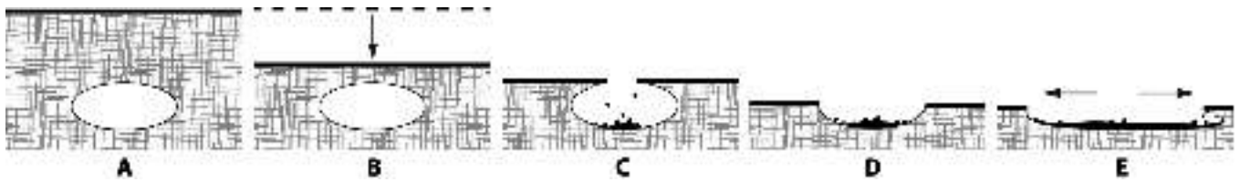
Fig. 17. Formation and evolution of the accumulation basins on Imhotep. A) Primordial void into the nucleus, resulting from its formation process. B) Progressive erosion of the surface and thinning down of the layer of material above the void. C) and D) collapse of the thin upper layer. E) Enlargement of the basin and infill with eroded material of the edges. Possible formation of overhangs.
