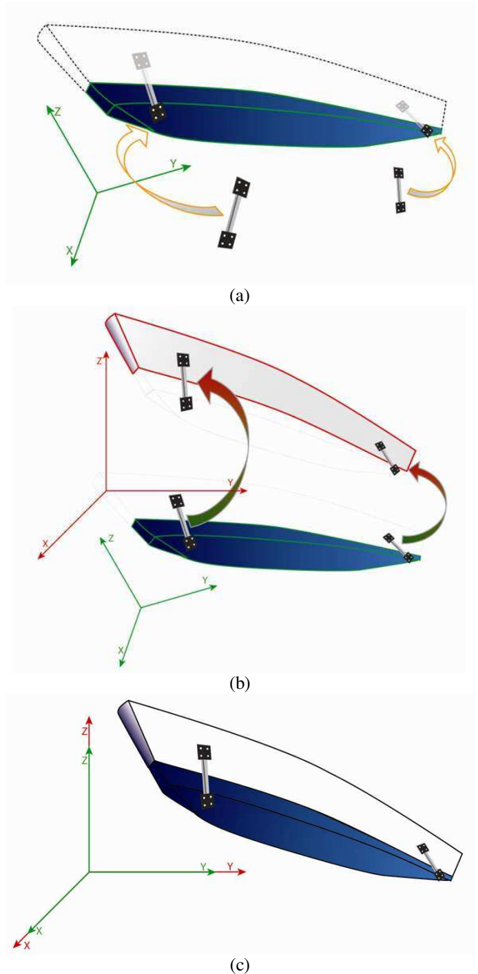
Figure 4 – Schematic procedure of the alignment of the two separate surveys above and below the waterline.
