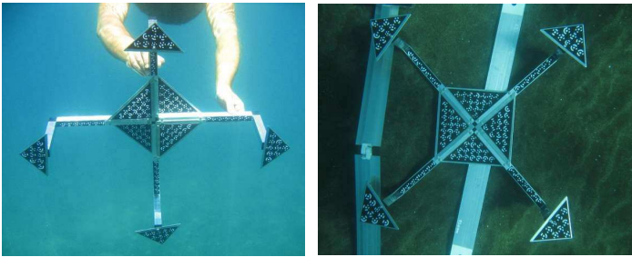
Figure 6. Two images used for the underwater calibrations of the Canon A620 in shallow water (left) and at a depth of 4m (right) respectively.
