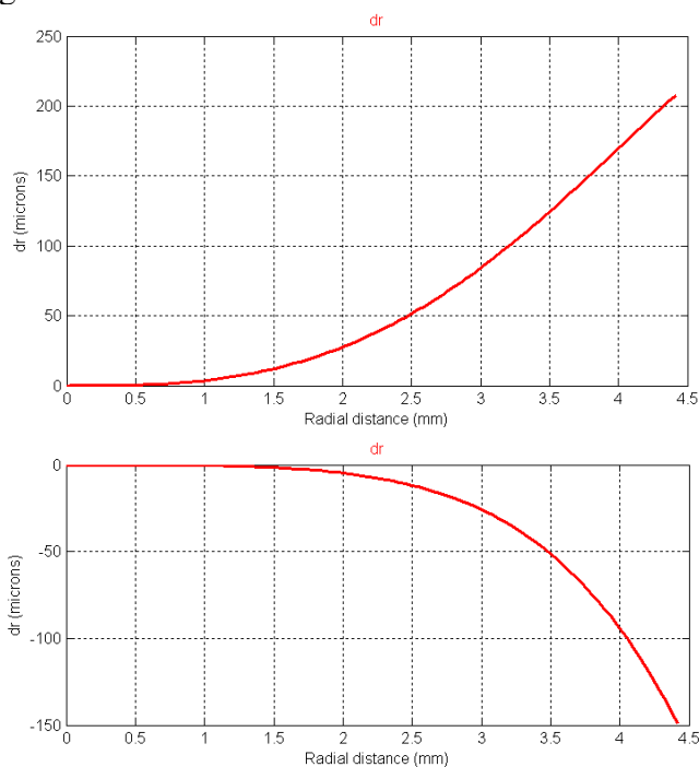
Figure 7. Radial distortion profiles for “dry” calibration (up) and underwater calibrations (down).
