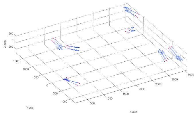
Figure 9. Residuals of the similarity transformation on the targets of the orientation devices.
