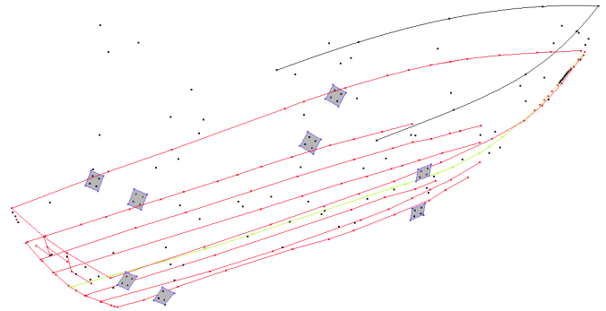
Figure 10. Feature lines and points measured in Photomodeler after the union of the two photogrammetric surveys.
