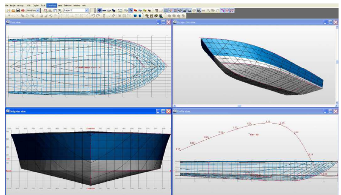
Figure 11. DELFT-ship model of Manò 19 .
