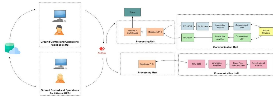
Figure 6. Ground Segment Overall Architecture
