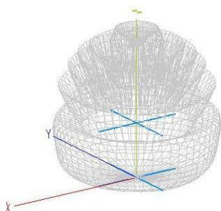
Figure 4. Turnstile Radiation Pattern
